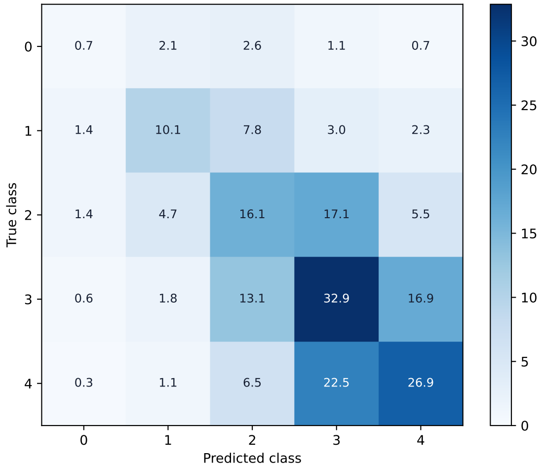
ROI Mask: mean confusion matrix over 15 runs
