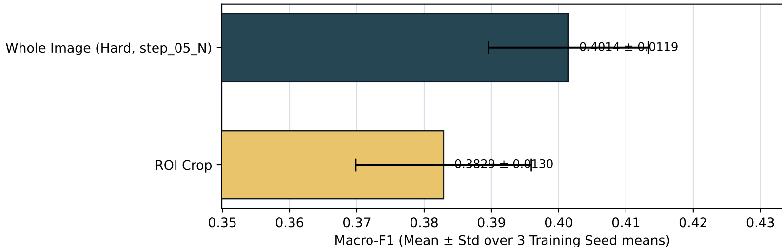
ROI Crop vs reference schemes (CEA five-class, N route) — Macro-F1 (5-fold CV, 3
