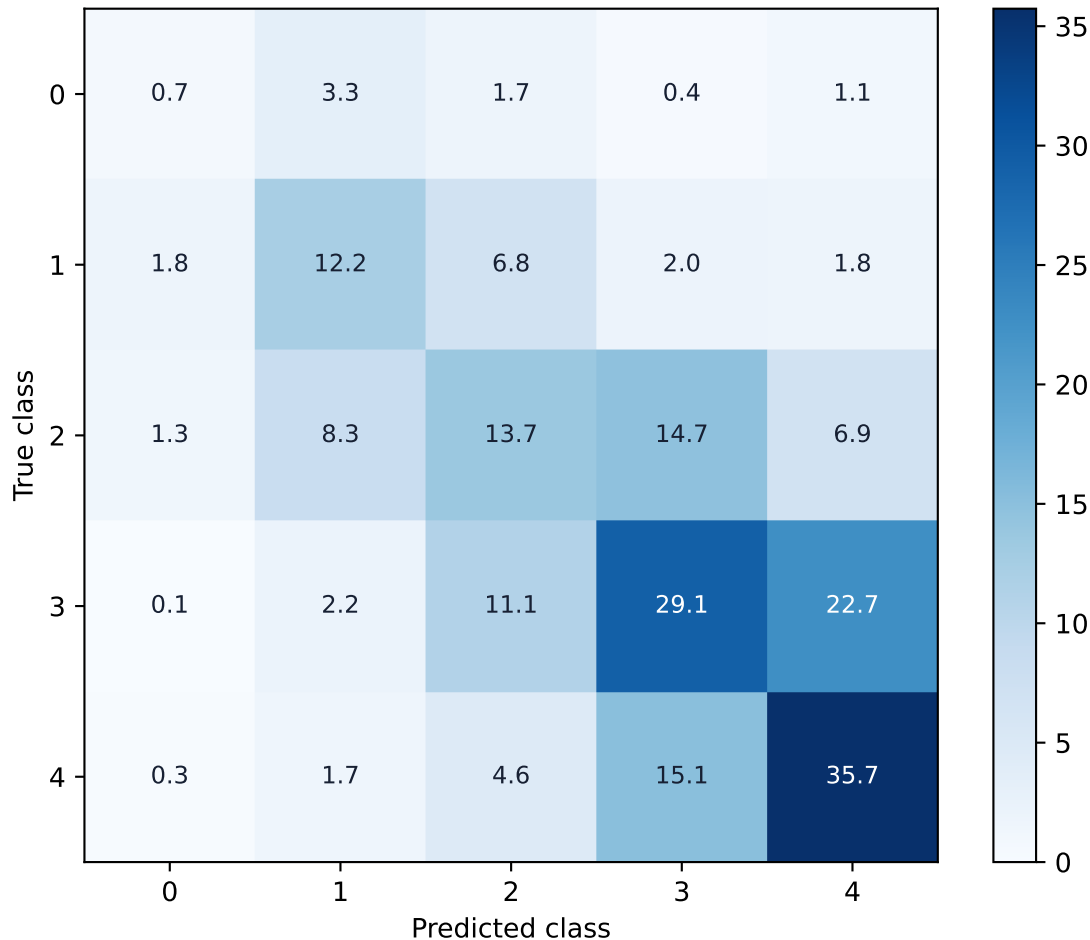
ROI Crop: mean confusion matrix over 15 runs
