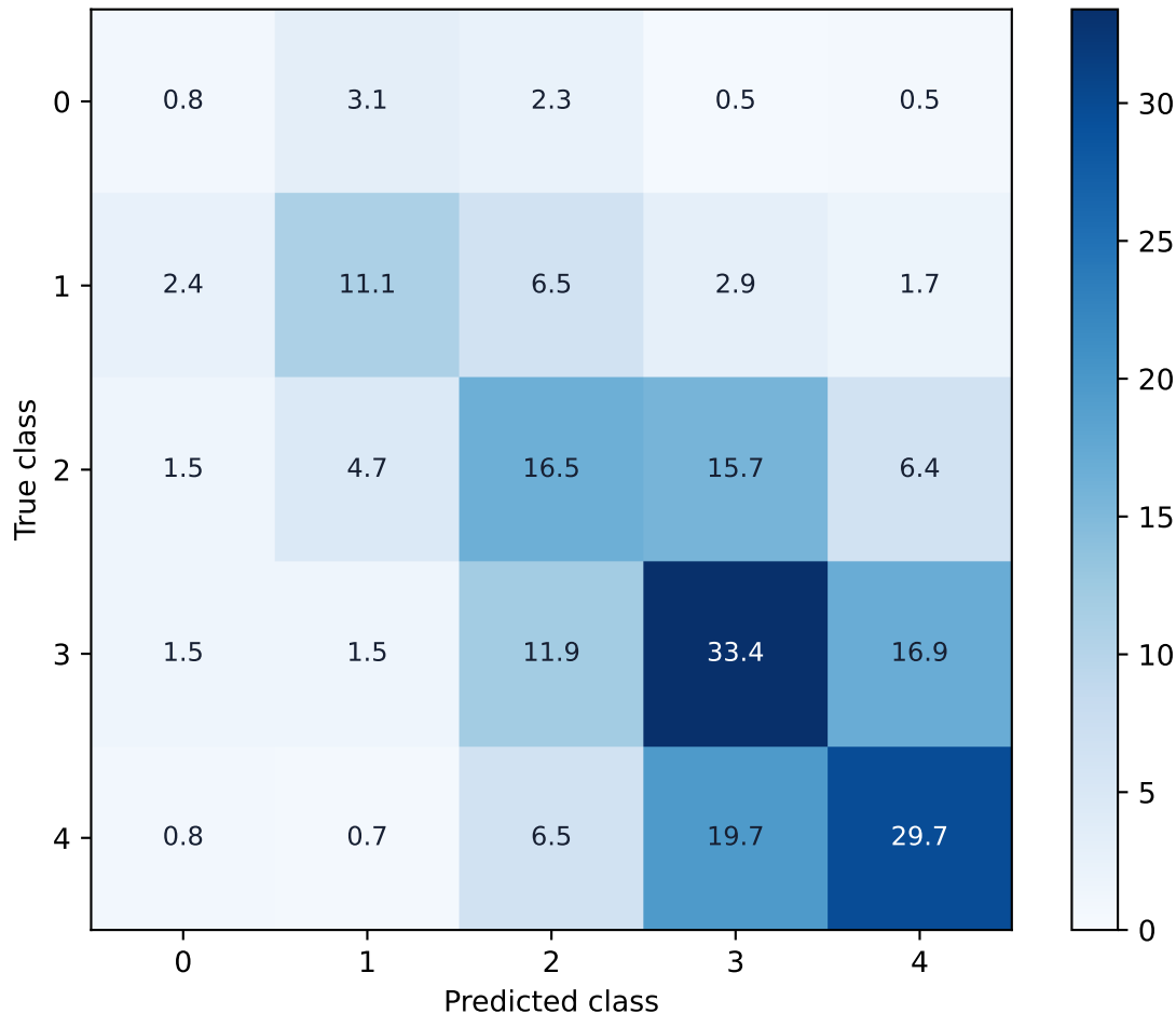
ROI + 20% Context: mean confusion matrix over 15 runs
