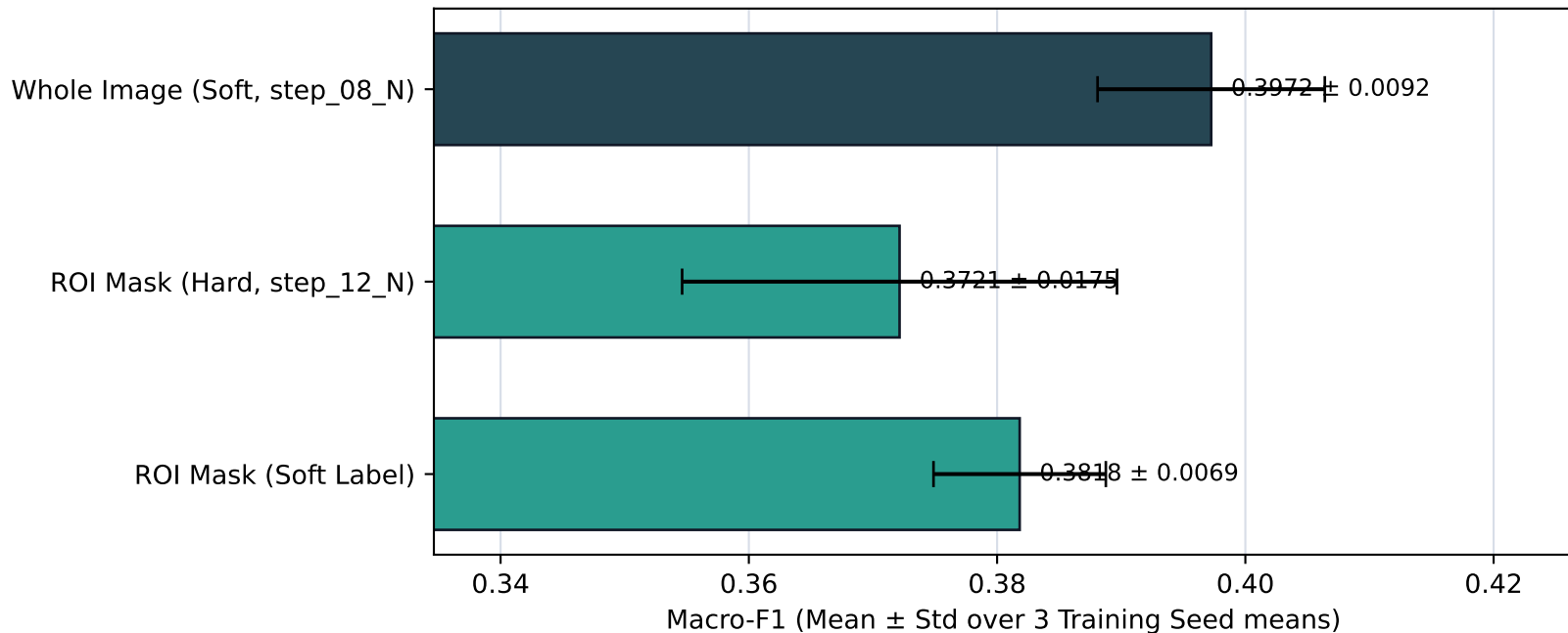
ROI Mask (Soft Label) vs reference schemes (CEA five-class, N route) — Macro-F1 (5-fold)
