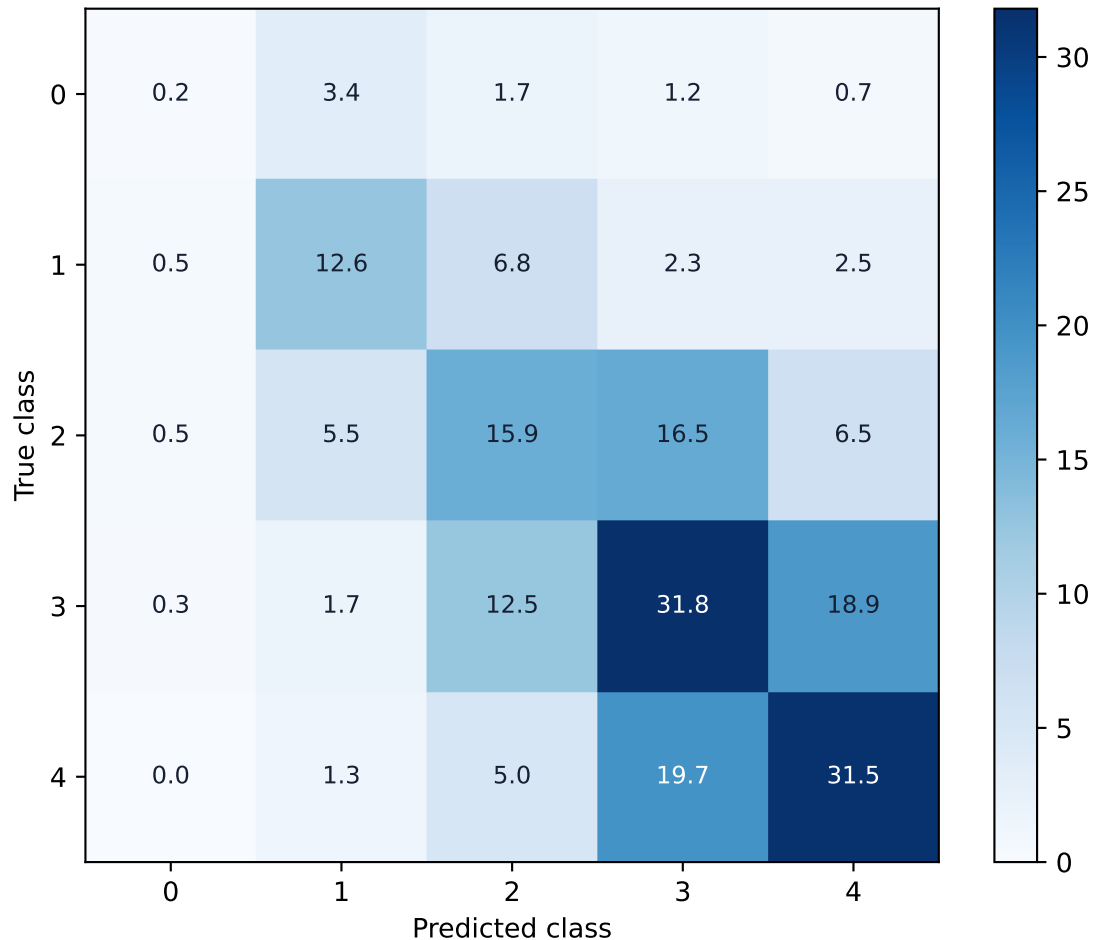
ROI Mask (Soft Label): mean confusion matrix over 15 runs
