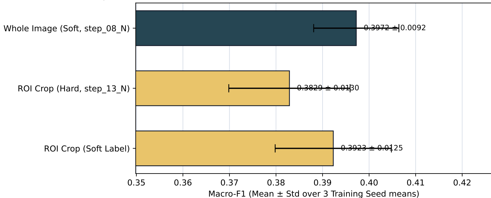
ROI Crop (Soft Label) vs reference schemes (CEA five-class, N route) — Macro-F1 (5-fold
