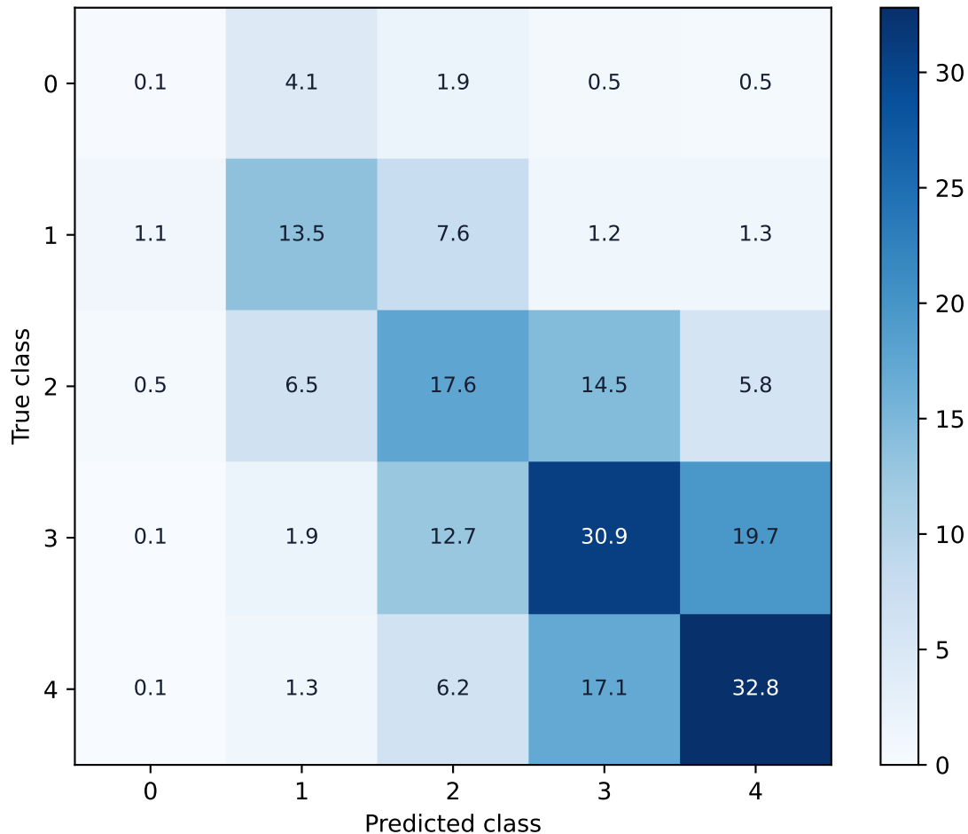
ROI Crop (Soft Label): mean confusion matrix over 15 runs
