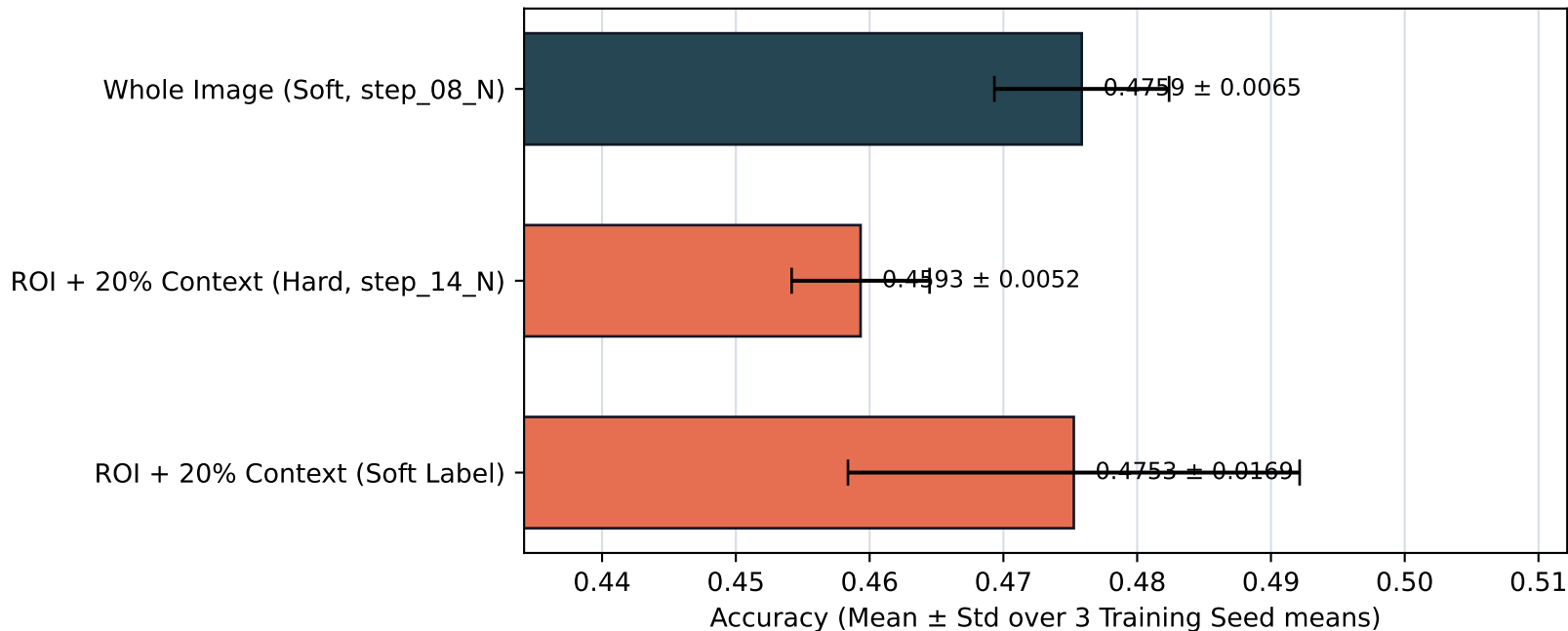
ROI + 20% Context (Soft Label) vs reference schemes (CEA five-class, N route) — Accuracy
