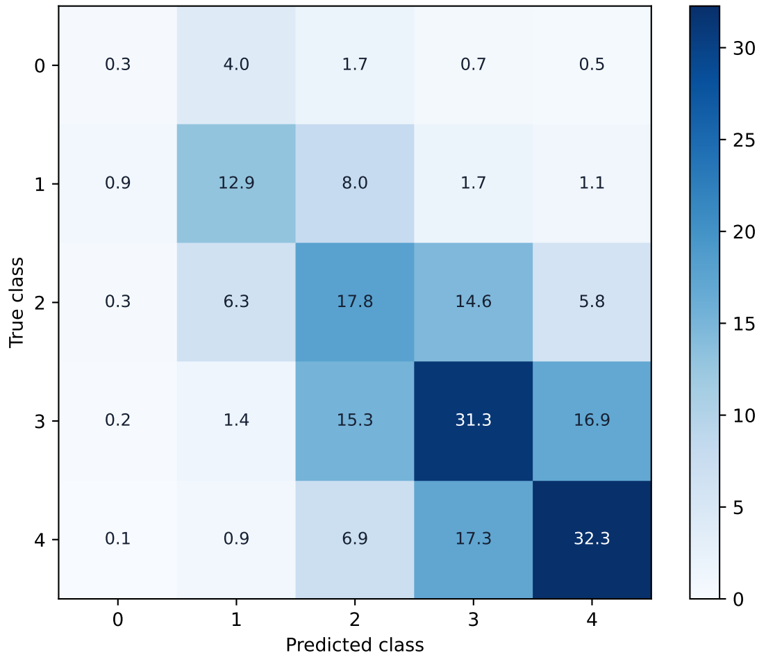
ROI + 20% Context (Soft Label): mean confusion matrix over 15 runs
