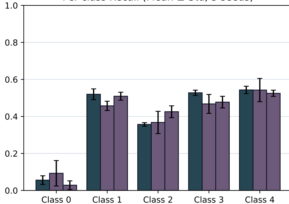
Per-class Recall (Mean \pm Std, 3 seeds)
