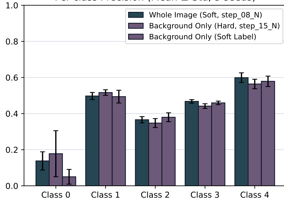
Per-class Precision (Mean \pm Std, 3 seeds)
