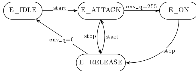
Figure 12: Attack/release envelope FSM in the PWM block. start is set by the 0x04 write and cleared by 0x08. Attack ramps the amplitude up, E_ON holds it, release ramps it down; a stop during attack or a start during release switches directly between the two ramps, so a retriggered tone never clicks.
