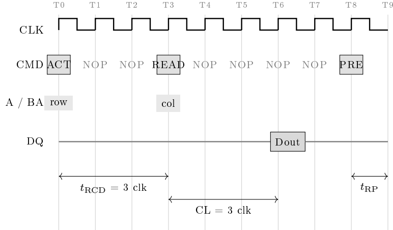
Figure 5: Start of an SDRAM read burst at 40.5 MHz (one clock = 24.7 ns). ACTIVATE at T0 opens the row, t_{RCD} later the READ at T3 selects the column, and with CAS latency 3 the first word is valid on DQ at T6 ( 3 \times 24.7 = 74 \text{ ns} after the READ). From there the burst continues, one word per clock, until the programmed data_len of 26 words is out; then the controller precharges and the row is closed, after which t_{RP} must elapse before the next ACTIVATE (in the figure the burst is cut short to fit the page).
