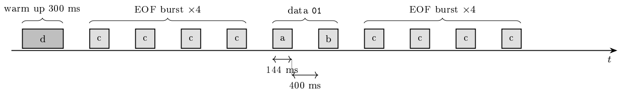
Figure 18: One transmission on the air (here the presence request, pattern 01). Every box is a two tone burst (carrier + data tone); the darker, longer first box is the warm up EOF that settles the receiver’s AGC. The receiver collapses each EOF burst into one EOF event by detection by change, so what reaches the protocol layer is exactly c 0 1 c .
