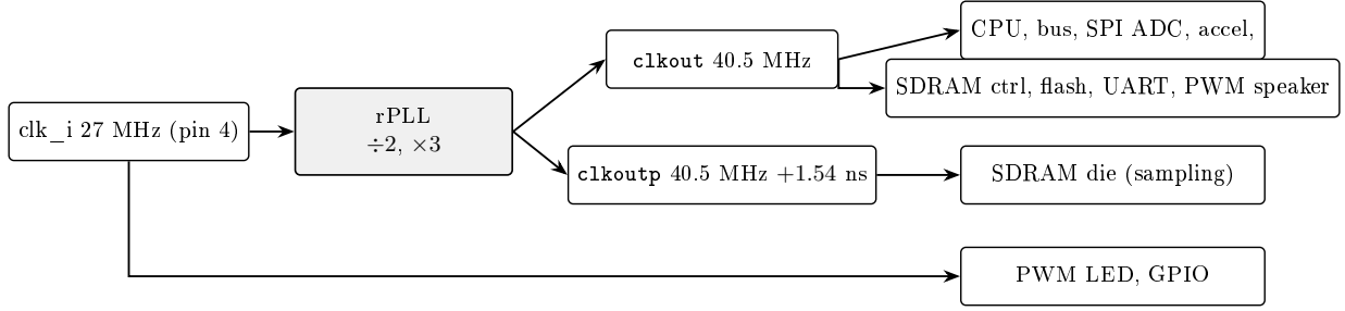
Figure 4: Clock tree. The 27MHz input is the PLL reference and also clocks the LED PWM and the GPIO directly. The rPLL produces 40.5 MHz ( clkout ) for the CPU, bus and most peripherals, including the speaker PWM (same domain as the bus, so no clock domain crossing on its registers), and a +1.54 ns phase shifted copy ( clkoutp ) that clocks only the SDRAM die.
