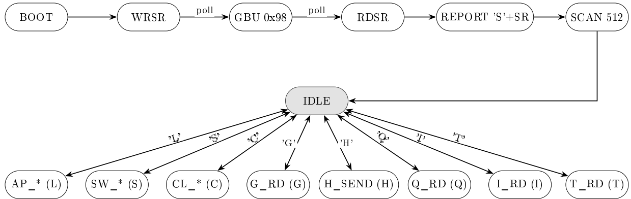
Figure 14: The storage state machine (drawn from flash_ctrl.vhd ; the firmware port keeps the same shape). At power up it unlocks the chip (WRSR clears the protection bits BP0..BP2 and SRP and sets QE, then a Global Block Unlock), reads the status register back, reports it unsolicited over the UART ('S' plus the SR byte; in practice the ESP32 boots too late to catch it and asks again with T), and scans all 512 slots to find the head of the ring buffer, then sits in IDLE. Each UART opcode (L append, S save settings, C clear, G read slots, H read head, Q read settings, I JEDEC id, T read status register) is entered from IDLE on its character and returns to IDLE when its SPI sequence finishes; the double headed arrows mean exactly that go and return.
