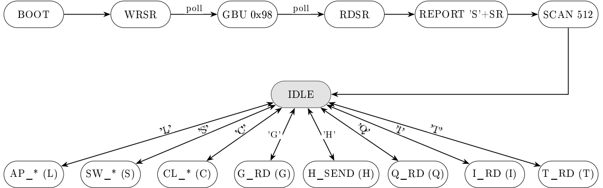
Figure 14: flash_ctrl state machine. At power up it unlocks the chip (WRSR clears the protection bits BP0..BP2 and SRP and sets QE, then a Global Block Unlock), reads the status register back, reports it unsolicited over the UART ('S' plus the SR byte; in practice the ESP32 boots too late to catch it and asks again with T), and scans all 512 slots to find the head of the ring buffer, then sits in IDLE. Each UART opcode (L append, S save settings, C clear, G read slots, H read head, Q read settings, I JEDEC id, T read status register) is entered from IDLE on its character and returns to IDLE when its SPI sequence finishes; the double headed arrows mean exactly that go and return.
