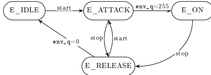
Figure 12: Attack/release envelope FSM in the PWM block. start is set by the 0x04 write and cleared by 0x08. Attack ramps the amplitude up, E_ON holds it, release ramps it down; a stop during attack or a start during release switches directly between the two ramps, so a retriggered tone never clicks.
