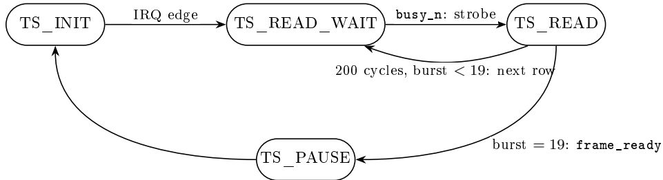
Figure 7: The fetch FSM. One loop iteration per burst: wait for the controller, strobe the read with the burst’s row address, collect words for a fixed 200 cycle window while rd_valid unloads into the BSRAM, then move to the next row. After burst 19 it signals the frame and re-arms for the next IRQ.
