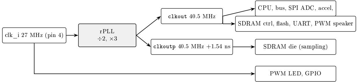
Figure 4: Clock tree. The 27 MHz input is the PLL reference and also clocks the LED PWM and the GPIO directly. The rPLL produces 40.5 MHz ( clkout ) for the CPU, bus and most peripherals, including the speaker PWM (same domain as the bus, so no clock domain crossing on its registers), and a +1.54 ns phase shifted copy ( clkoutp ) that clocks only the SDRAM die.
