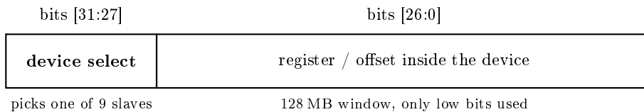
Figure 3: The 32 bit address is split in two. The top five bits addr[31:27] pick the slave (Table 2); the low 27 bits are the offset inside that slave, of which each peripheral decodes only the few it needs (the per device register maps below).
