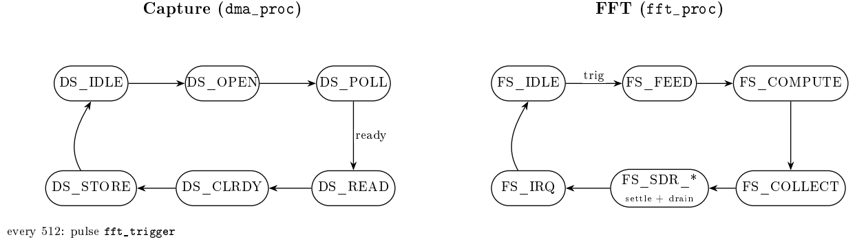
Figure 9: The two parallel FSMs. Capture reads one ADC sample per pass ( DS_OPEN starts the SPI, DS_POLL waits for the conversion, DS_READ/DS_STORE write it into the ping-pong buffer) and pulses fft_trigger every 512 samples. The FFT FSM, on that trigger, feeds the window ( FS_FEED ), runs the FFT ( FS_COMPUTE ), collects the bins ( FS_COLLECT ), then takes ownership of the SDRAM write port and drains them ( FS_SDR_* : the settle guard, then warm up plus 20 row bursts) and raises the IRQ ( FS_IRQ ), after which it also streams the frame on a debug pin before re-arming. The two FSMs cannot collide: capture’s only shared resource is the Wishbone bus (M1, to reach the ADC), while the drain uses the dedicated SDRAM port and never touches the bus.
