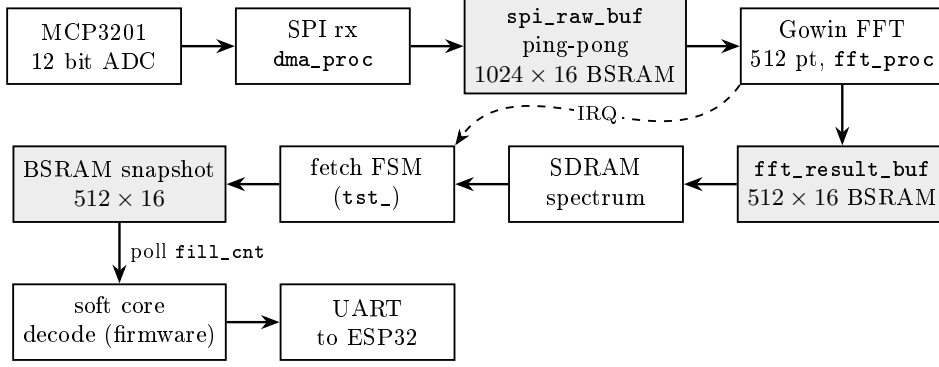
Figure 8: Receive pipeline (black and white). The capture FSM fills one half of the ping-pong block RAM while the FFT FSM processes the other half into a spectrum in SDRAM, through the controller’s dedicated write port. The frame done IRQ (dashed) starts the fetch FSM, which copies the spectrum into the stable BSRAM snapshot; the soft core polls the snapshot counter over the bus (S0), copies the 512 bins and, in firmware, decodes one character per tone and sends it to the ESP32.
