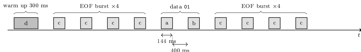
Figure 16: One transmission on the air (here the presence request, pattern 01). Every box is a two tone burst (carrier + data tone); the darker, longer first box is the warm up EOF that settles the receiver’s AGC. The receiver collapses each EOF burst into one EOF event by detection by change, so what reaches the protocol layer is exactly c 0 1 c .
