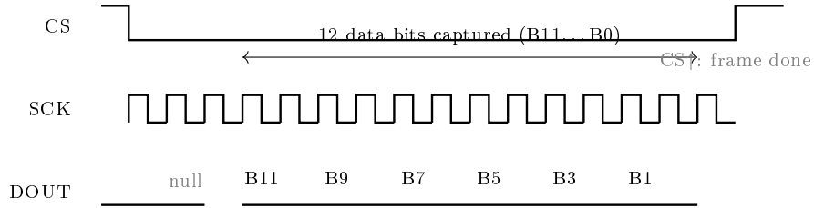
Figure 10: MCP3201 read as seen by the SPI master. CS goes low, the master issues 16 SCK periods at 750 kHz, discards the leading null bit, captures the 12 data bits B11 down to B0 most significant first, then raises CS to end the frame. One frame is 16/750\text{ kHz} = 21.3\text{ }\mu\text{s} , which sets the 46.9 kHz sample rate.
