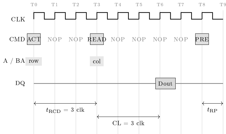
Figure 5: Start of an SDRAM read burst at 40.5 MHz (one clock = 24.7 ns). ACTIVATE at T0 opens the row, t_{RCD} later the READ at T3 selects the column, and with CAS latency 3 the first word is valid on DQ at T6 ( 3 \times 24.7 = 74\ \text{ns} after the READ). From there the burst continues, one word per clock, until the programmed data_len of 26 words is out; then the controller precharges and the row is closed, after which t_{RP} must elapse before the next ACTIVATE (in the figure the burst is cut short to fit the page).
