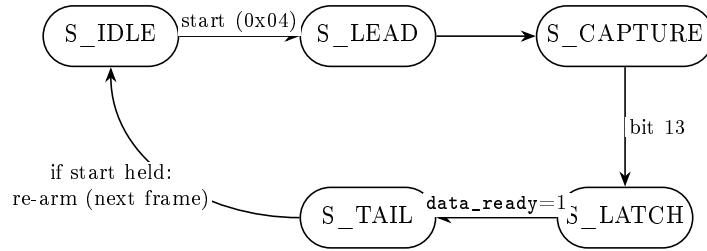
Figure 11: SPI master (ADC) frame FSM, from spi_master.vhd . A write to 0x04 asserts CS low and starts one MCP3201 frame of 16 SCK periods at 750 kHz ( PRESCALER=54 from the 40.5 MHz clock). S_LEAD clocks the leading null bit, S_CAPTURE shifts MISO in most significant first for the 12 data bits, S_LATCH writes them into the 0x00 register and sets data_ready , S_TAIL raises CS to close the 21.3\text{ }\mu\text{s} frame. While 0x04 (start) stays asserted the frame re-arms, which gives the continuous 46.9 kHz sample stream the FFT needs; a write to 0x0C clears data_ready .
