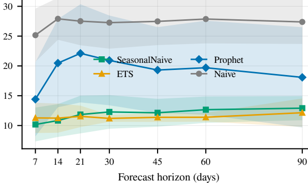
Walk-forward MAPE (%)
