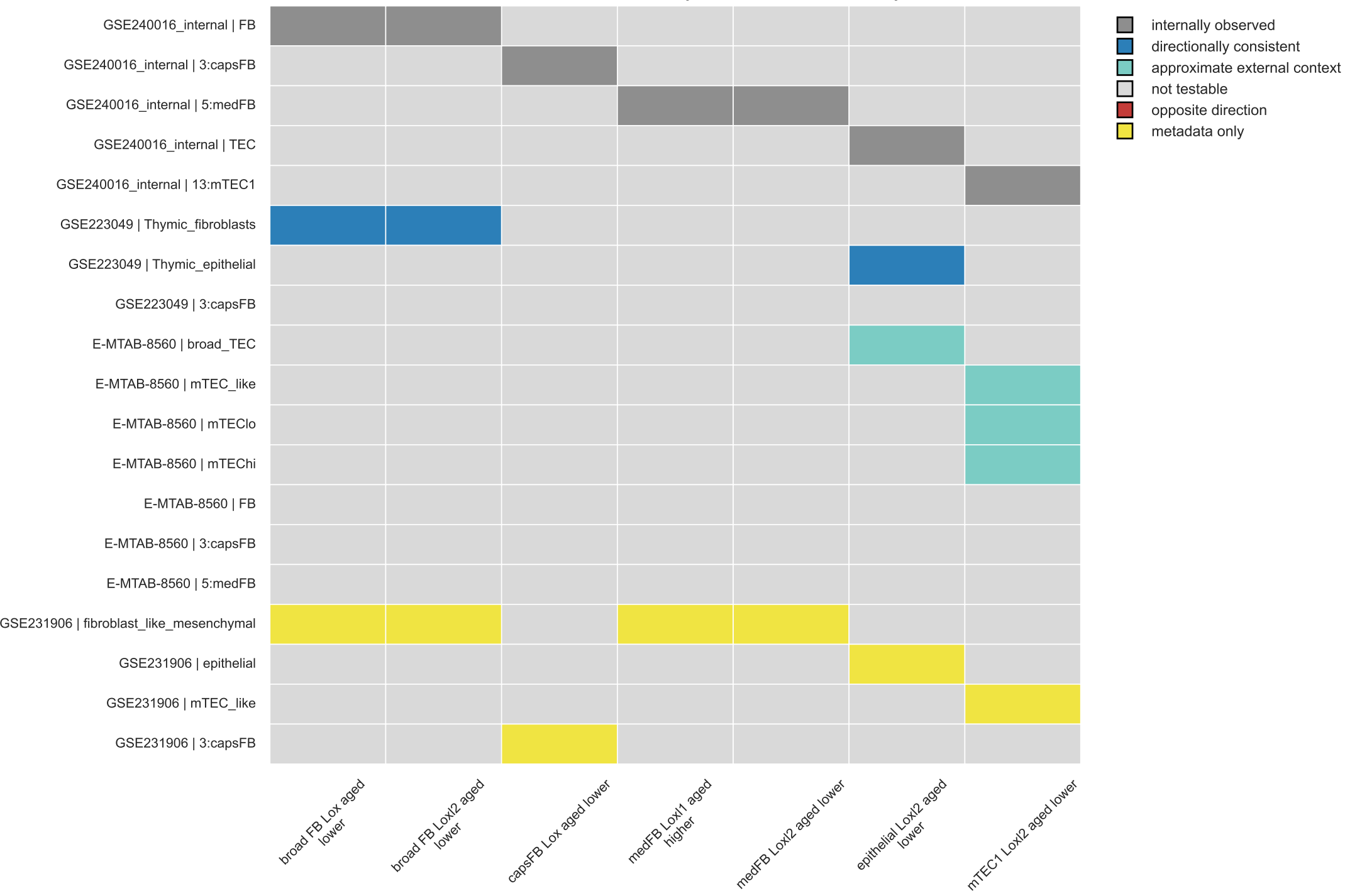
Cross-dataset LOX-family direction consistency
