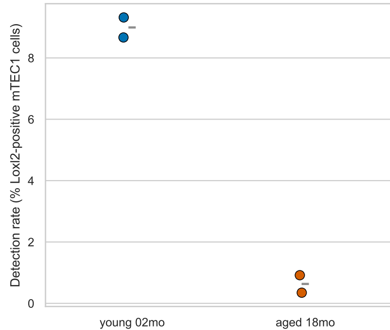
Detection
