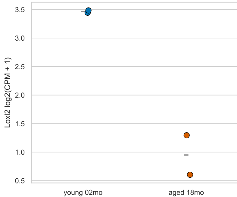
Expression
