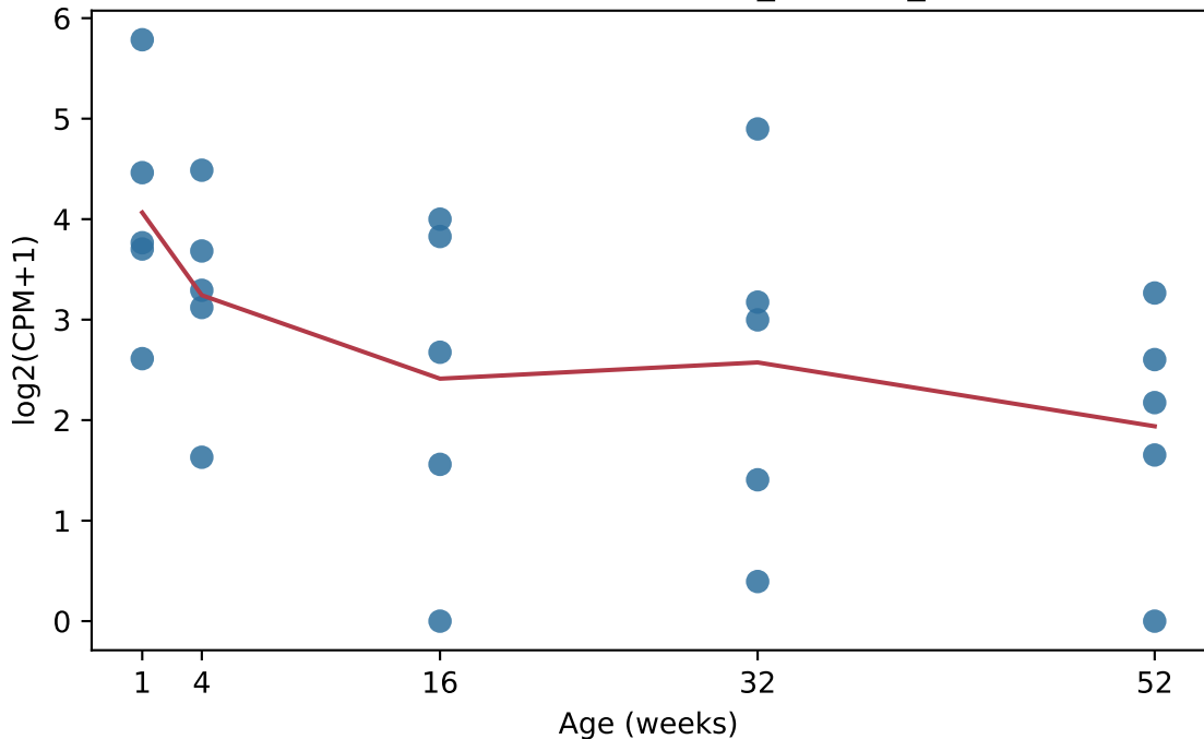
E-MTAB-8560 Loxl2 combined_mTEClo_mTEChi
