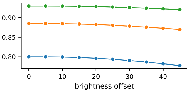
Contrast Decrease
