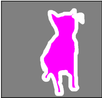
Ground Truth
