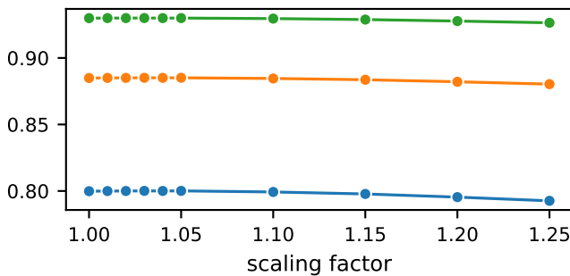
Gaussian Noise
