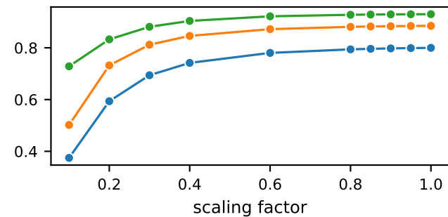
Gaussian Blur
