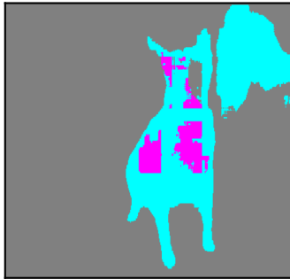
Predicted Mask
