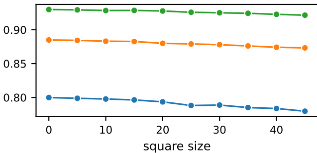
Occlusion
