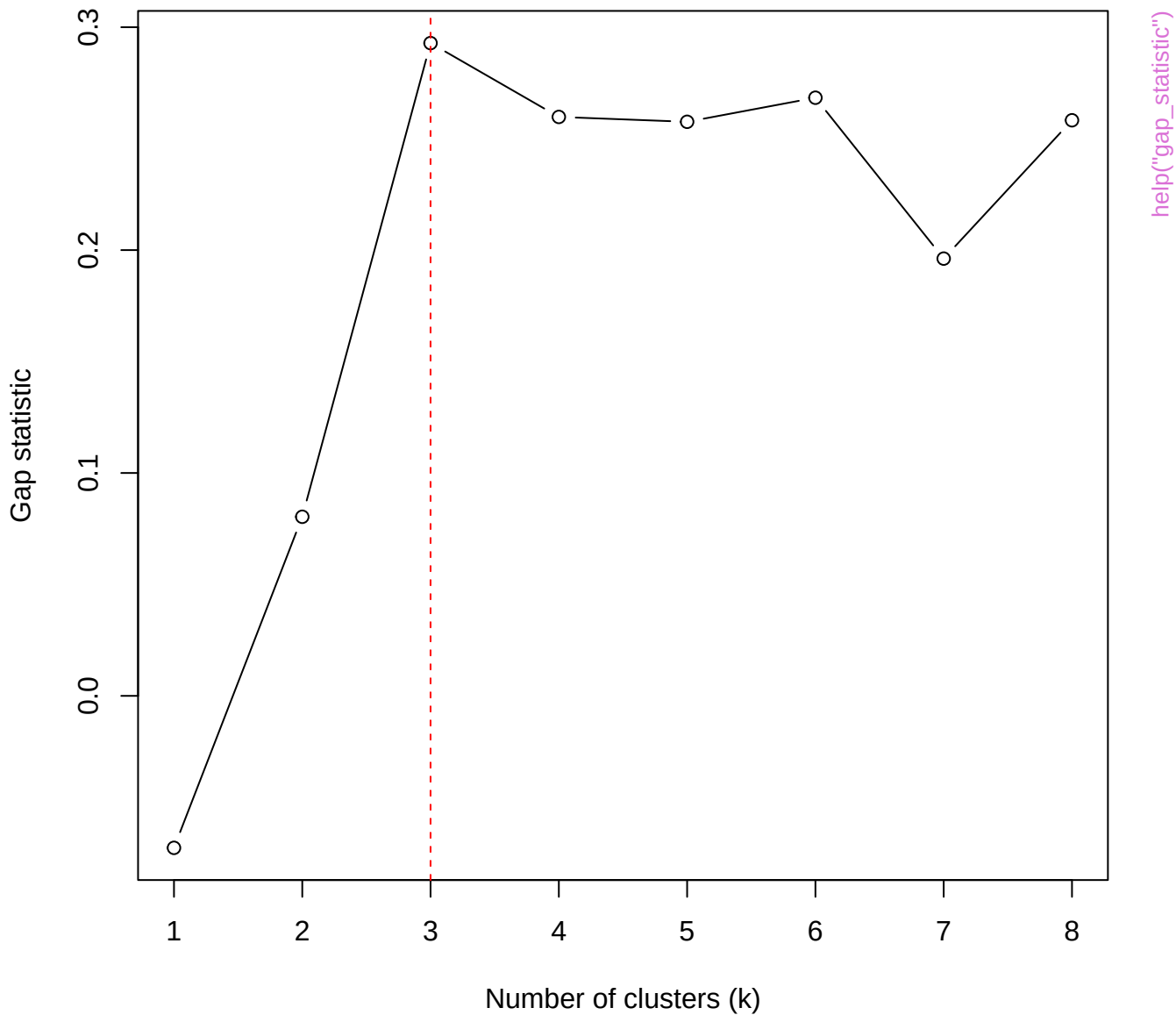
Gap Statistic for Optimal k
