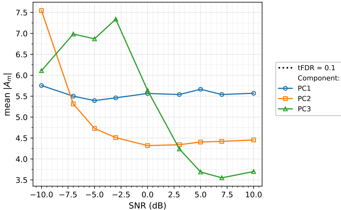
Selected support size
