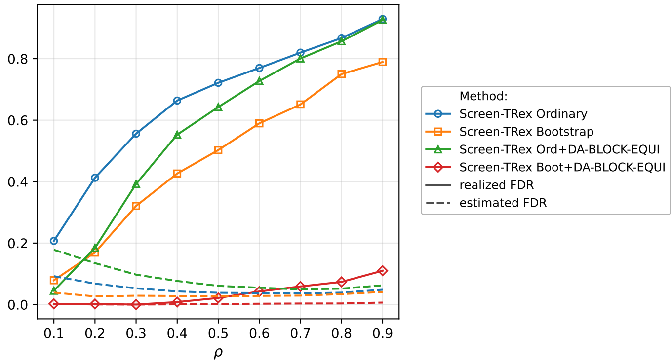
FDR: realized (solid) vs. estimated (dashed)
