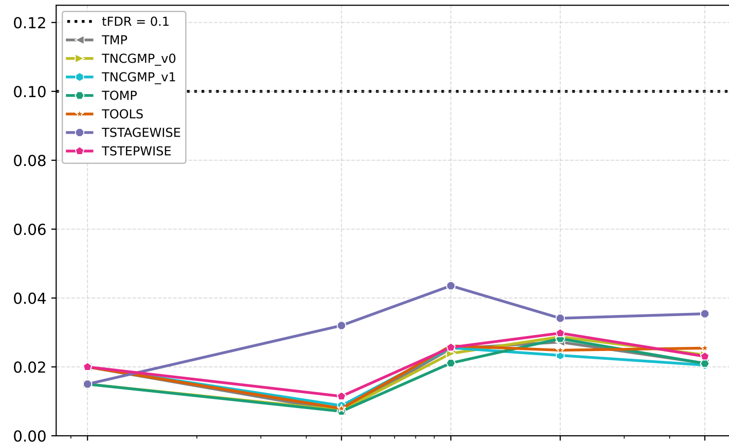
Method 8-14
