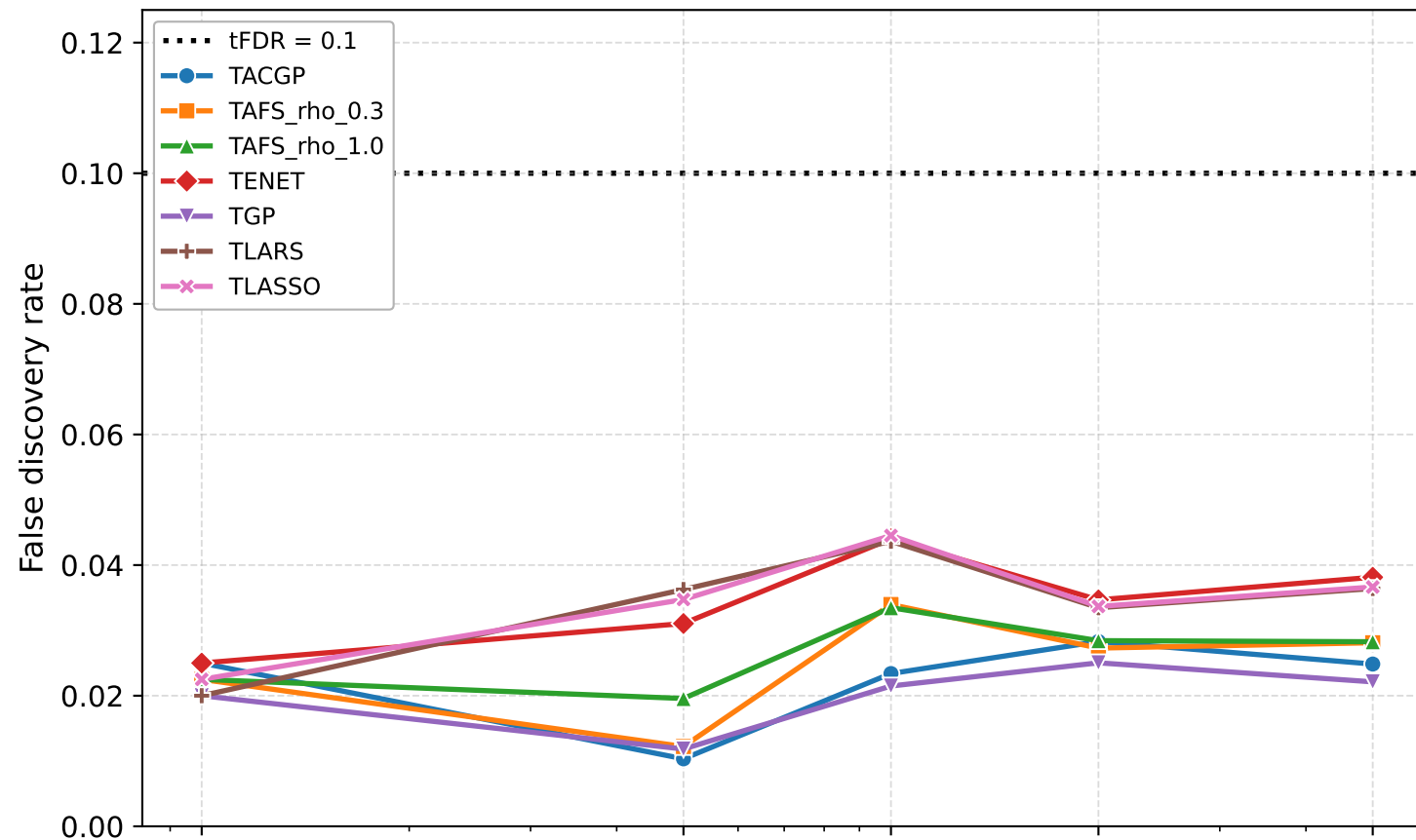
Method 1-7
