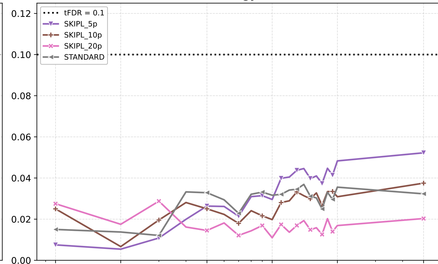
L-strategy 5-8
