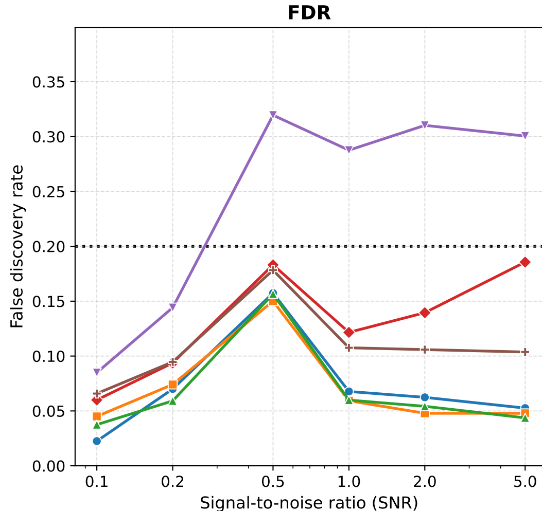
DA-TREx+AR1 vs base T-Rex on AR(1): SNR sweep at \rho = 0.7 (Random support)
