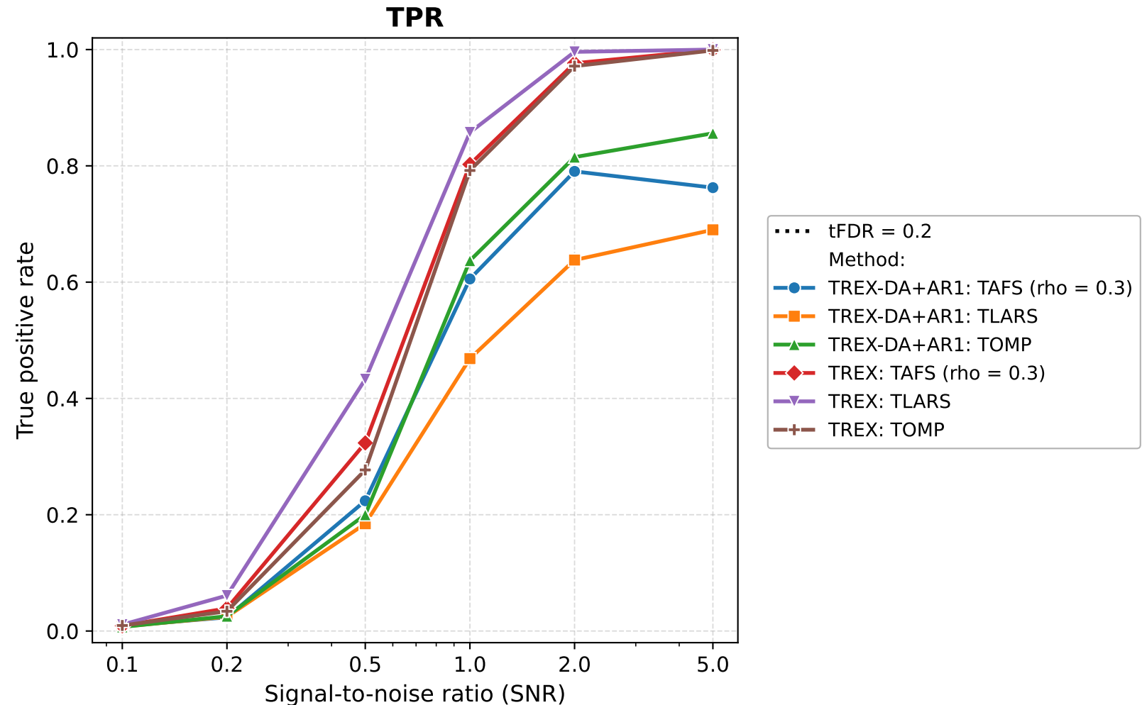
DA-TREx+AR1 vs base T-Rex on AR(1): SNR sweep at \rho = 0.7 (Random support)
