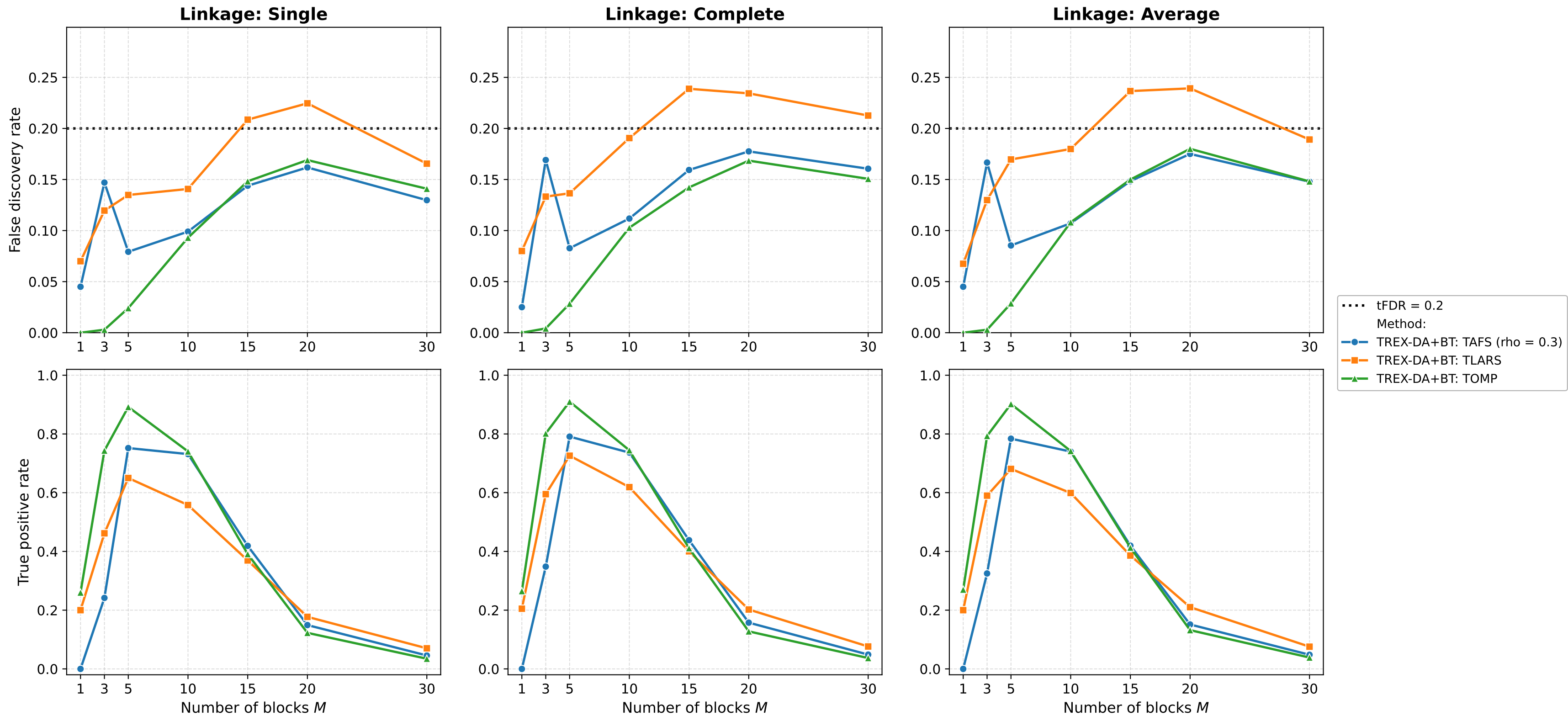
DA-Trex+BT, heavy-tailed: number-of-blocks M sweep across HAC linkage (Gaussian noise)
