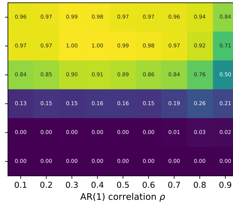
TREX-DA+NN: TAFS (rho = 0.3) TPR (true positive rate)
