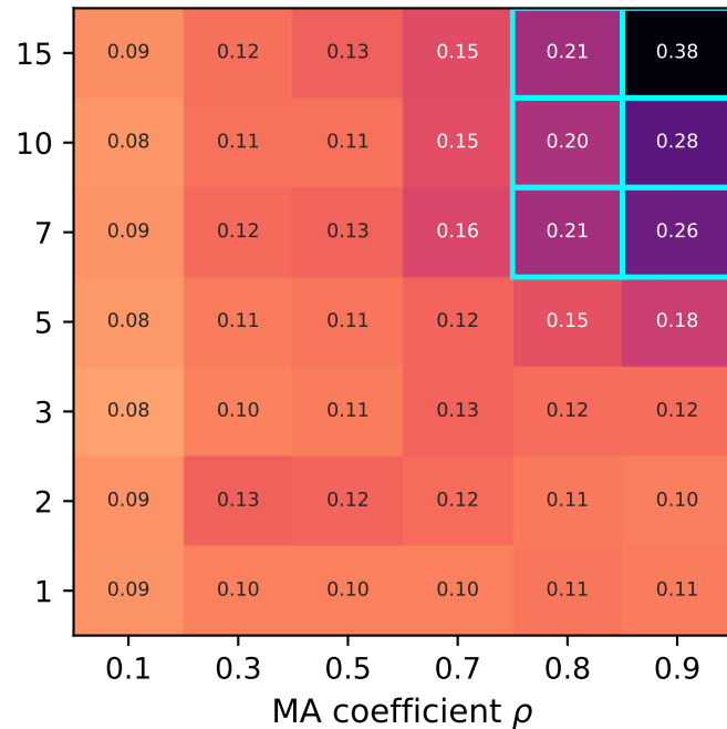
FDR (false discovery rate)
