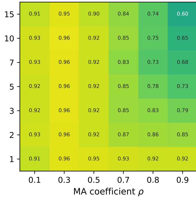
TREX-DA+NN: TLARS TPR (true positive rate)
