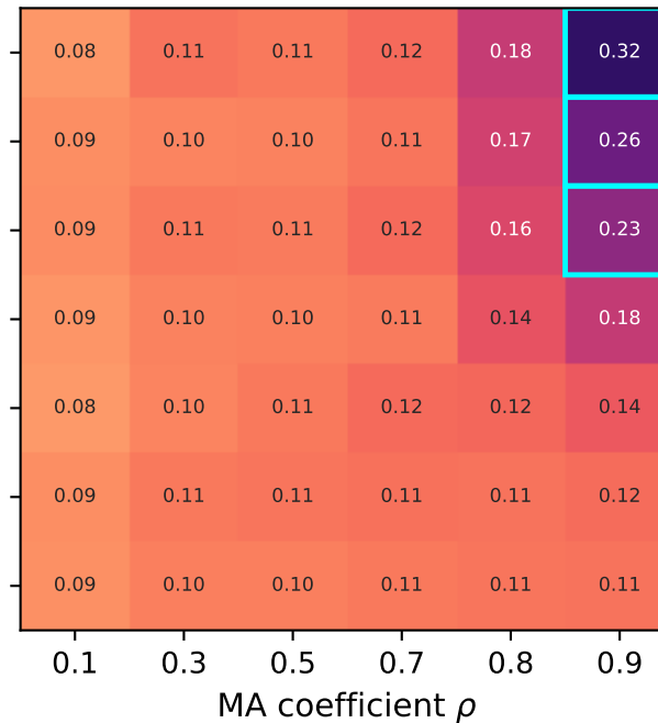
FDR (false discovery rate)
