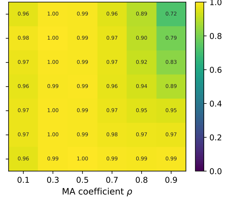
TREX-DA+NN: TOMP TPR (true positive rate)
