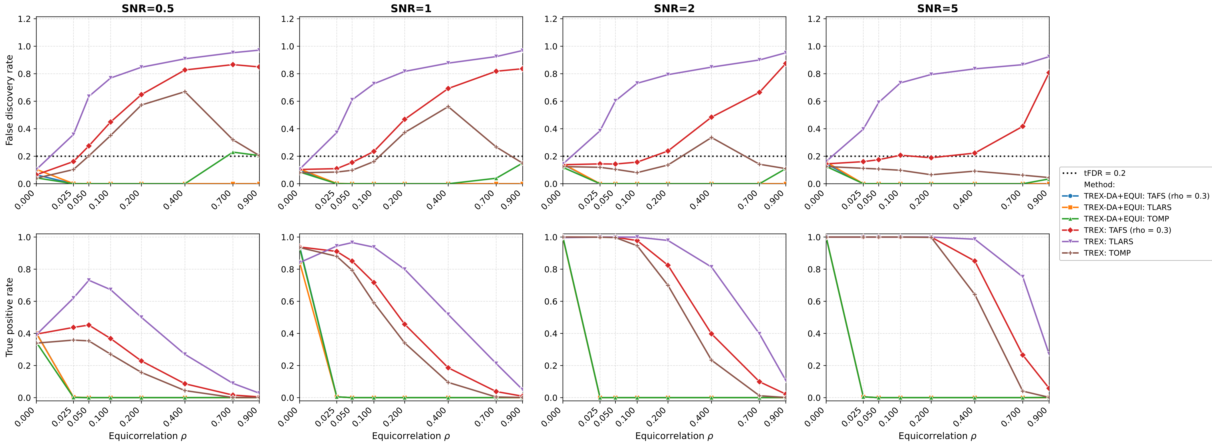
DA-Trex+EQUI vs base T-Rex on Equi: \rho sweep by SNR (Random support)
