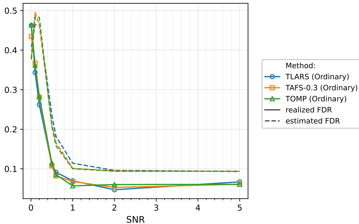
FDR: realized (solid) vs. estimated (dashed)
