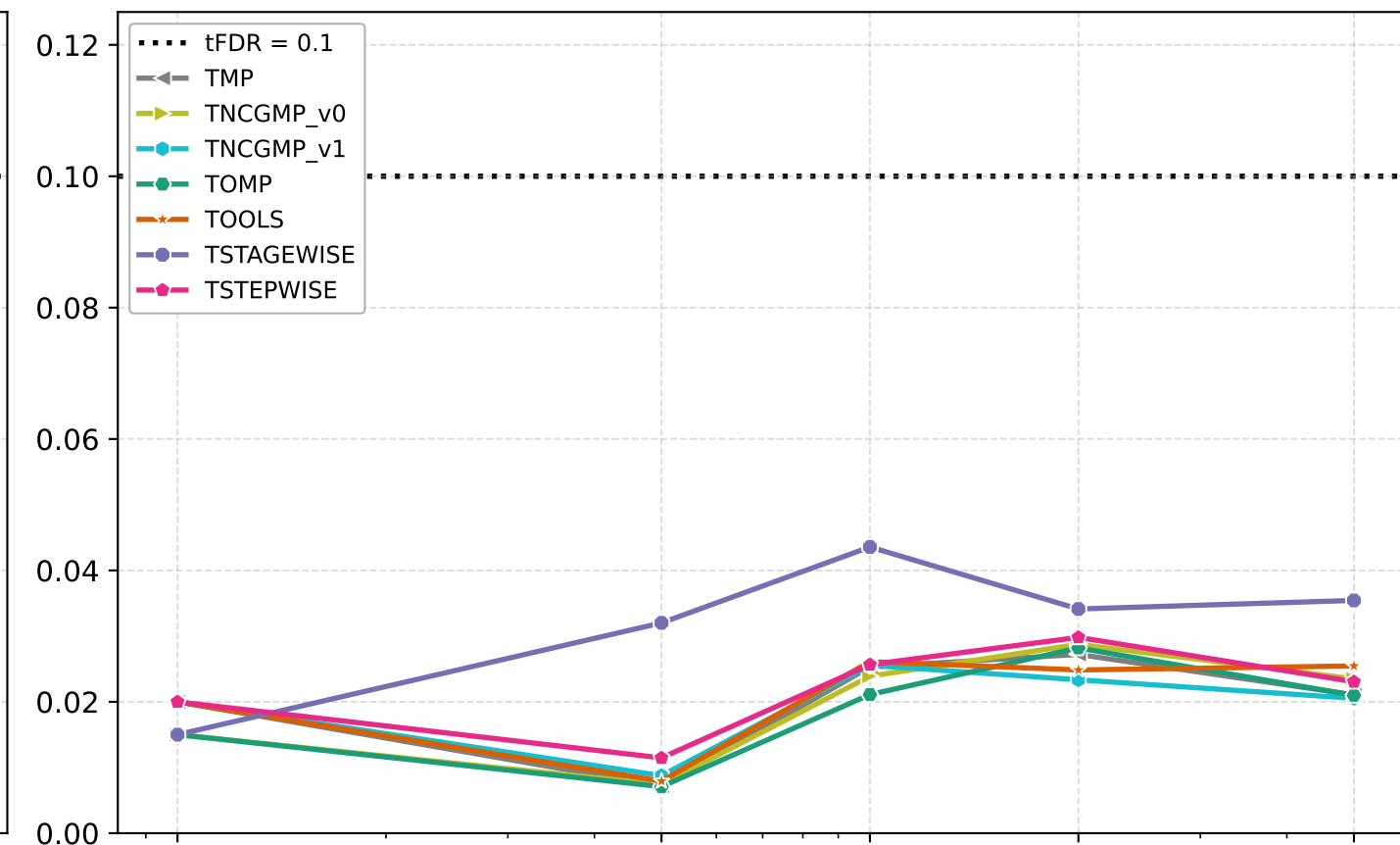
Solver 8-14
