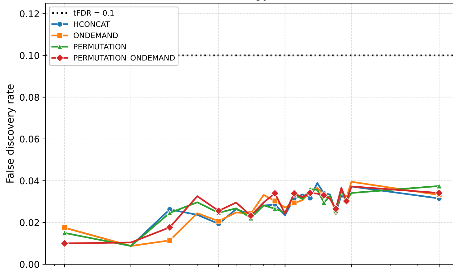
L-strategy 1-4
