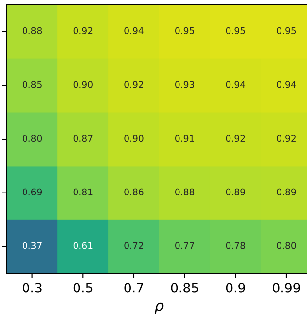
TENET_AUG TPR (true positive rate)
