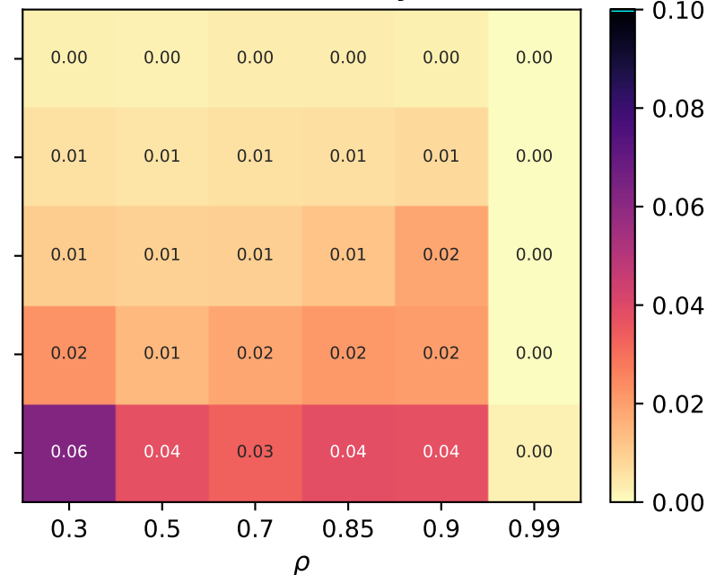
FDR (false discovery rate)
