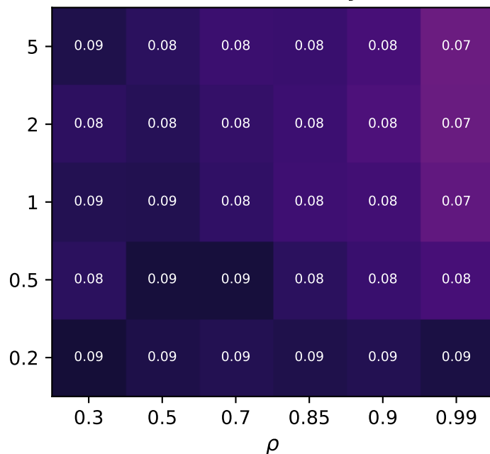
FDR (false discovery rate)
