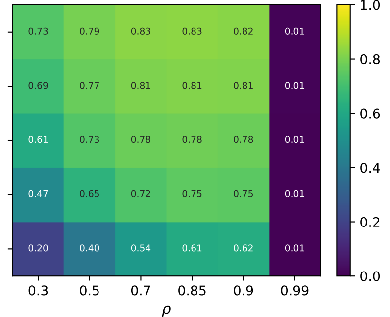
TIENET_AUG TPR (true positive rate)
