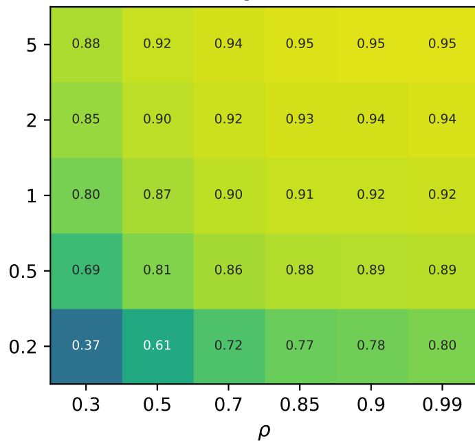
TENET TPR (true positive rate)
