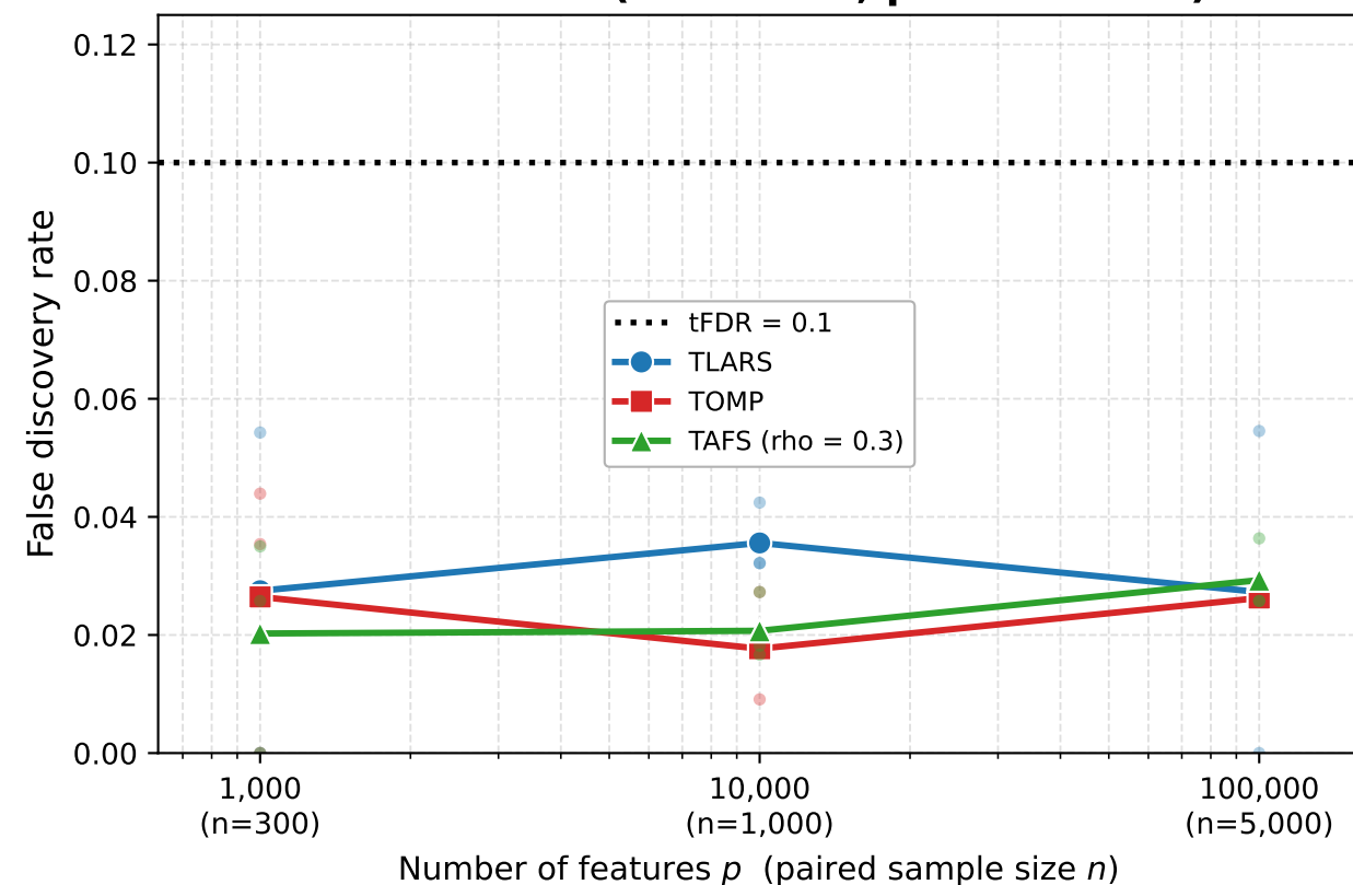
FDR at scale (mean line, per-SNR dots)
