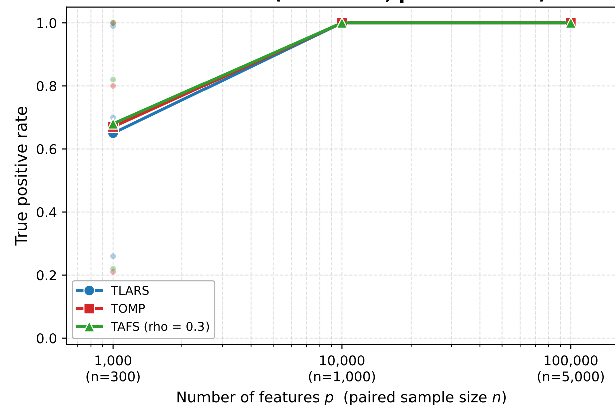
TPR at scale (mean line, per-SNR dots)
