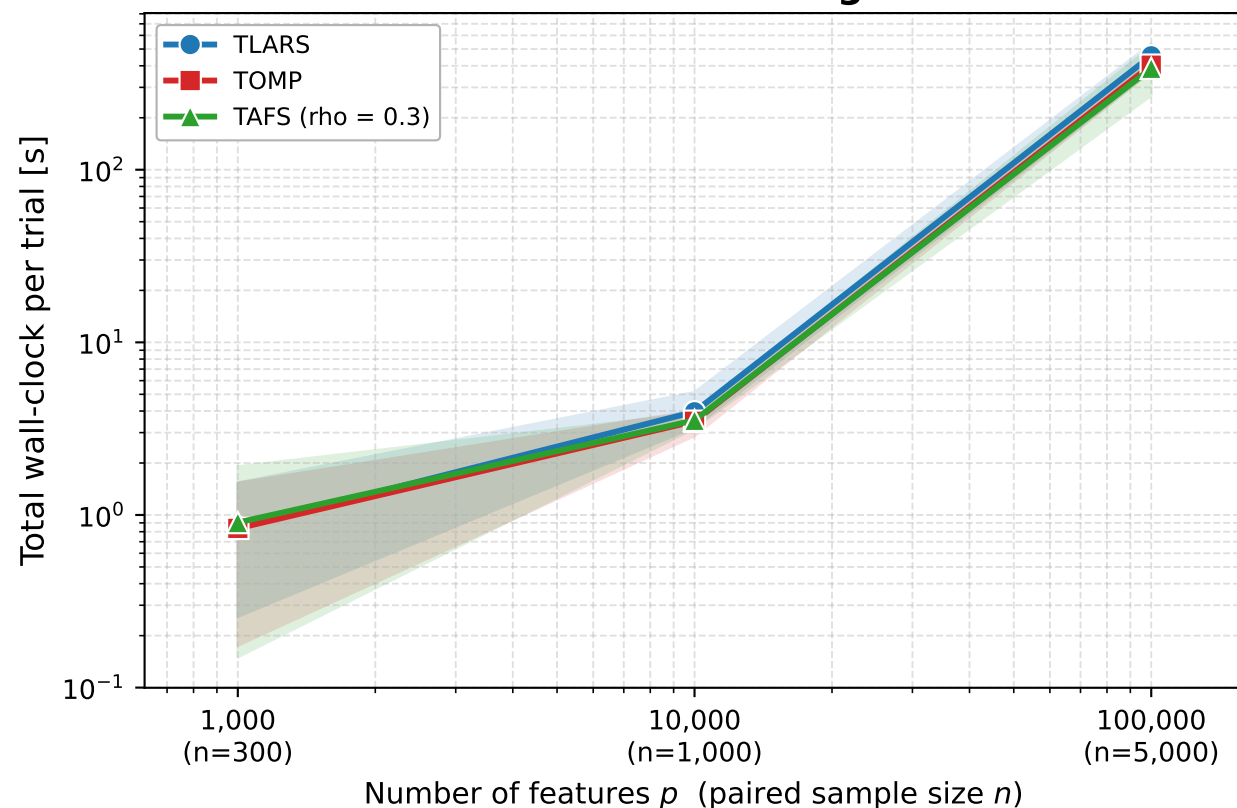
Runtime scaling
