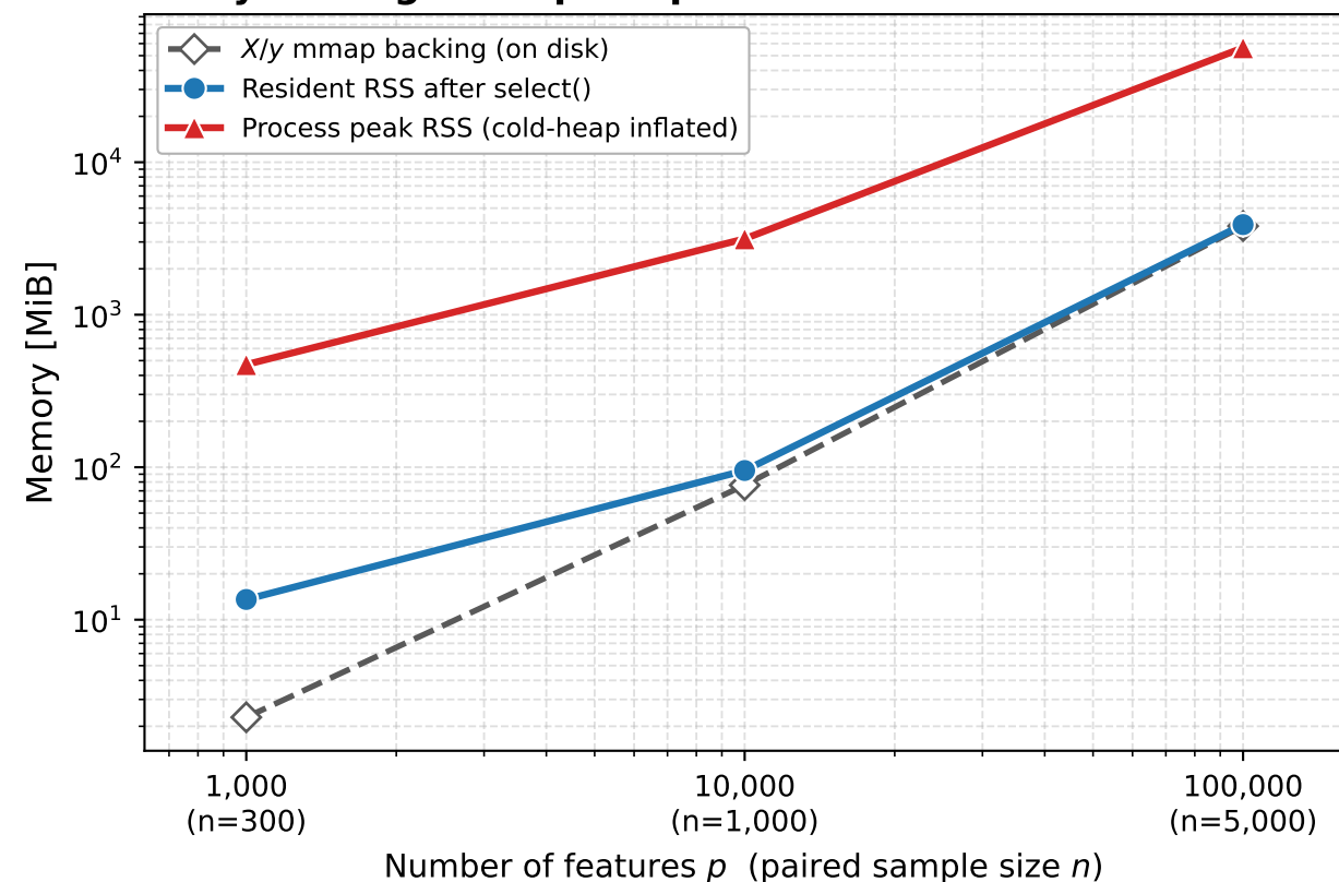
Memory scaling: mmap keeps resident RSS near the data size
