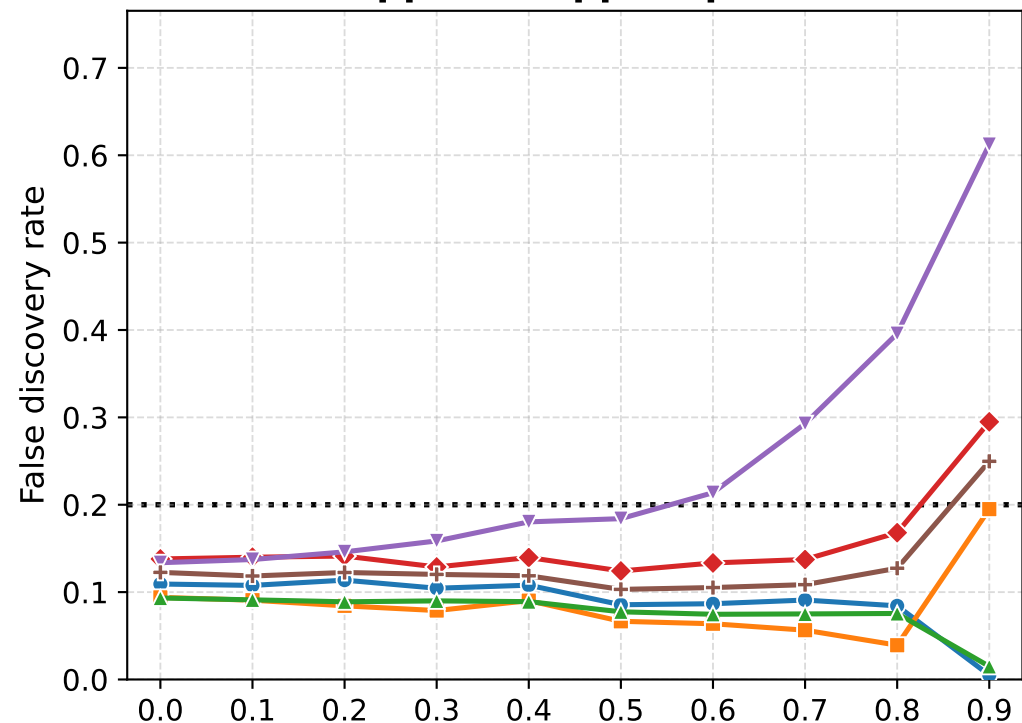
Support: CappedSpread
