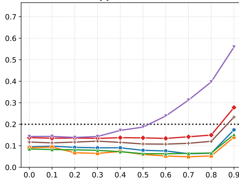
Support: Random
