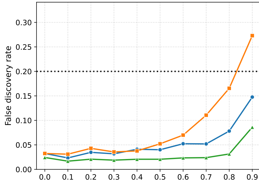
Noise: Gaussian
