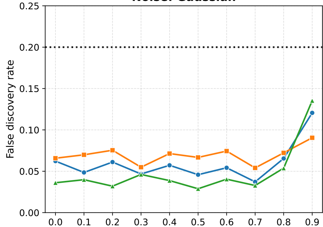
Noise: Gaussian
