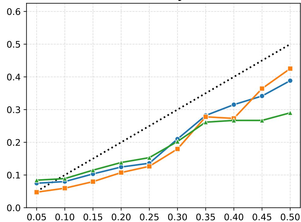
Noise: Heavy-tailed
