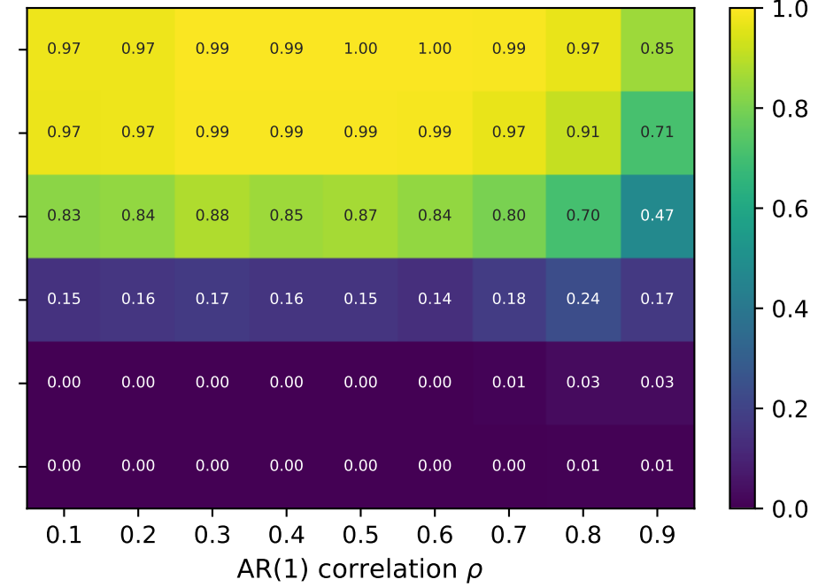
TREX-DA+NN: TOMP TPR (true positive rate)
