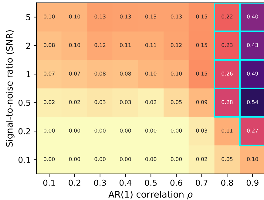
FDR (false discovery rate)
