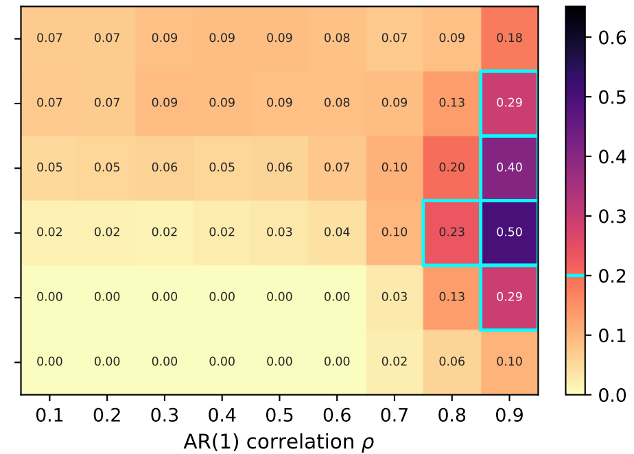
FDR (false discovery rate)
