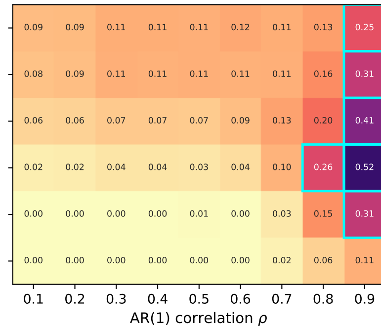
FDR (false discovery rate)
