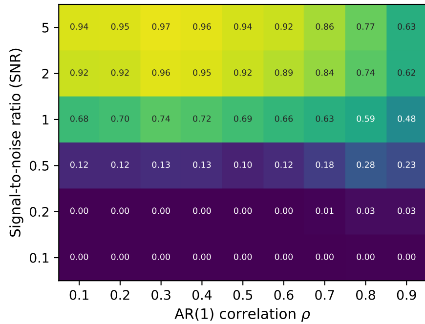
TREX-DA+NN: TLARS TPR (true positive rate)
