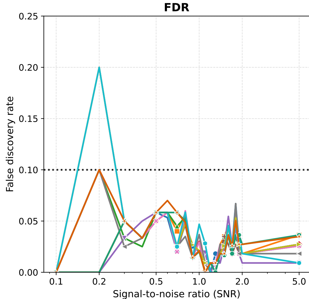
T-Rex dummy distributions ( n = 300 , p = 1000 , random support, 10 runs, TAFS + STANDARD)
