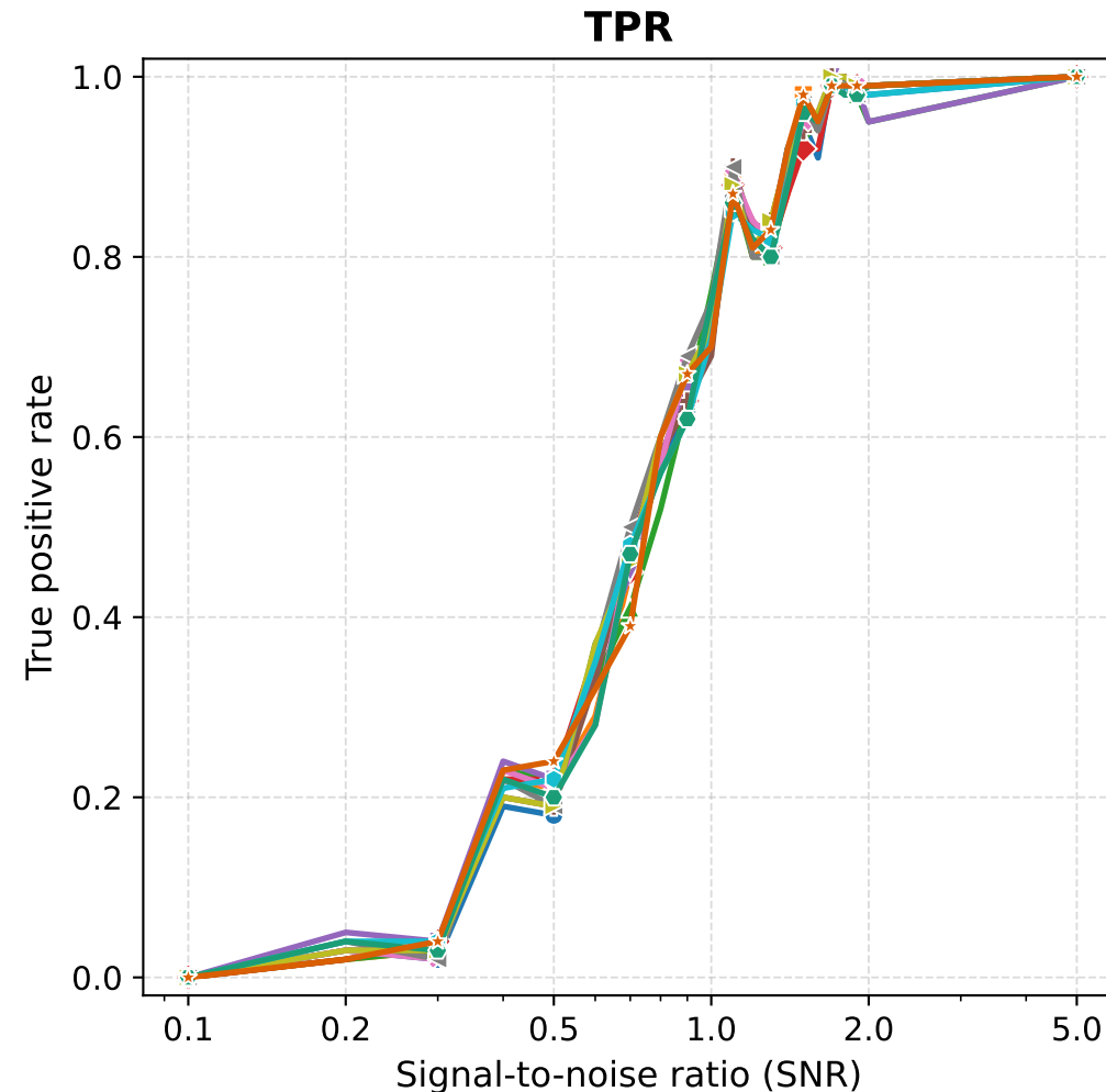
T-Rex dummy distributions ( n = 300 , p = 1000 , random support, 10 runs, TLARS + STANDARD)
