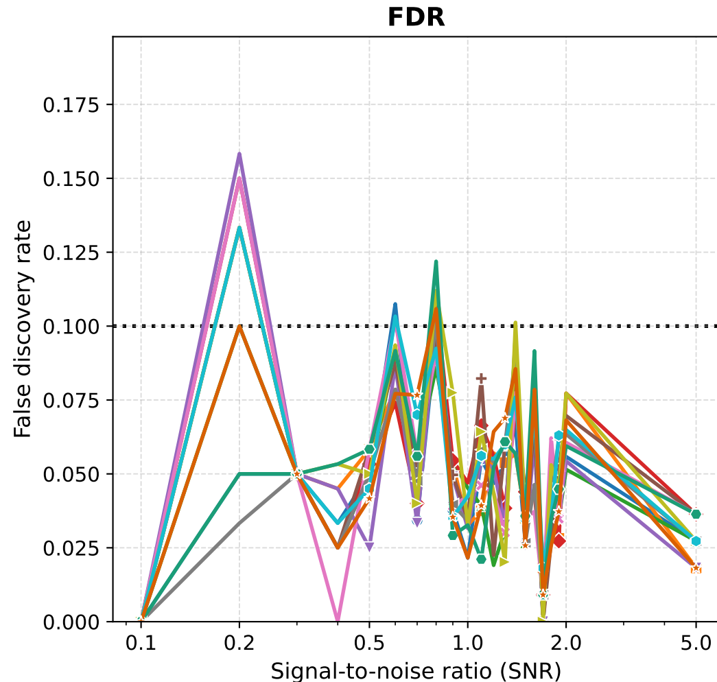
T-Rex dummy distributions ( n = 300 , p = 1000 , random support, 10 runs, TLARS + STANDARD)
