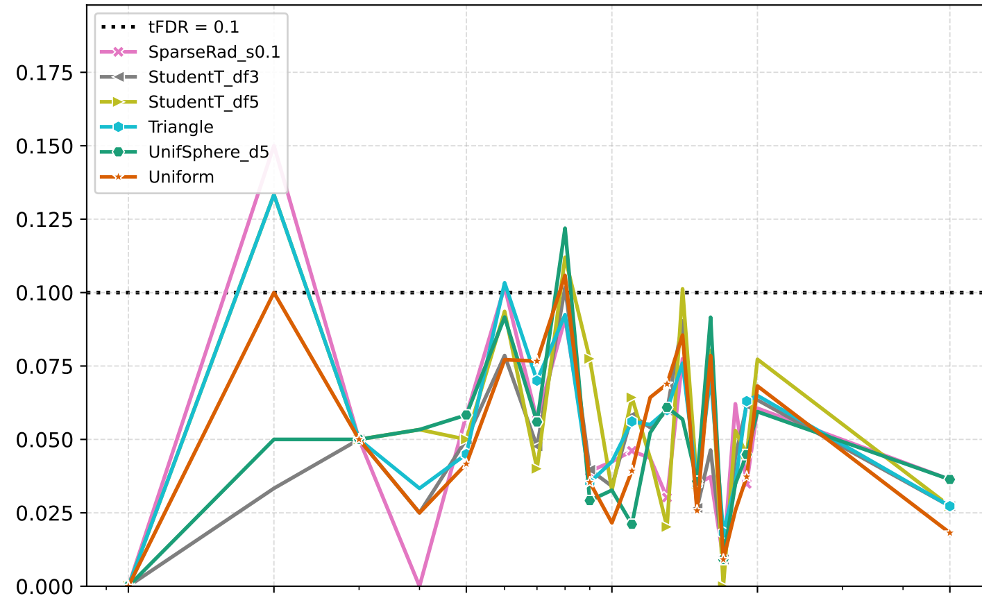
Dummy distribution 7-12
