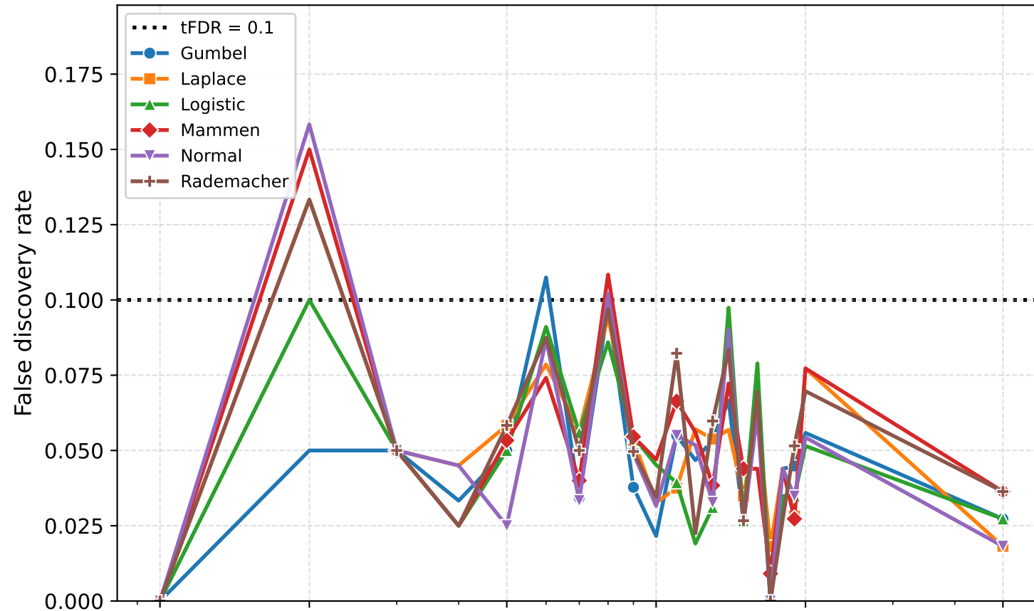
Dummy distribution 1-6
