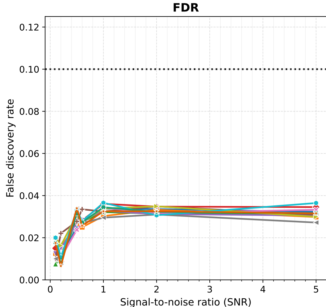
T-Rex dummy distributions ( n = 300 , p = 1000 , random support, TAFS ( \rho = 0.3 ) + STANDARD)
