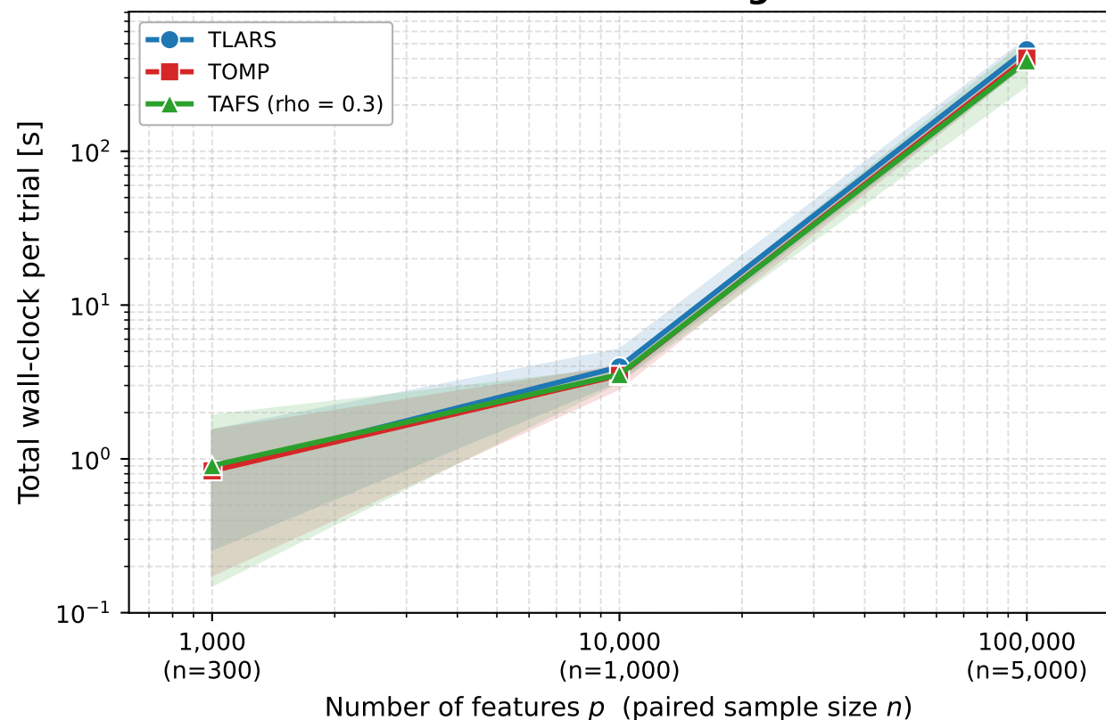
Runtime scaling
