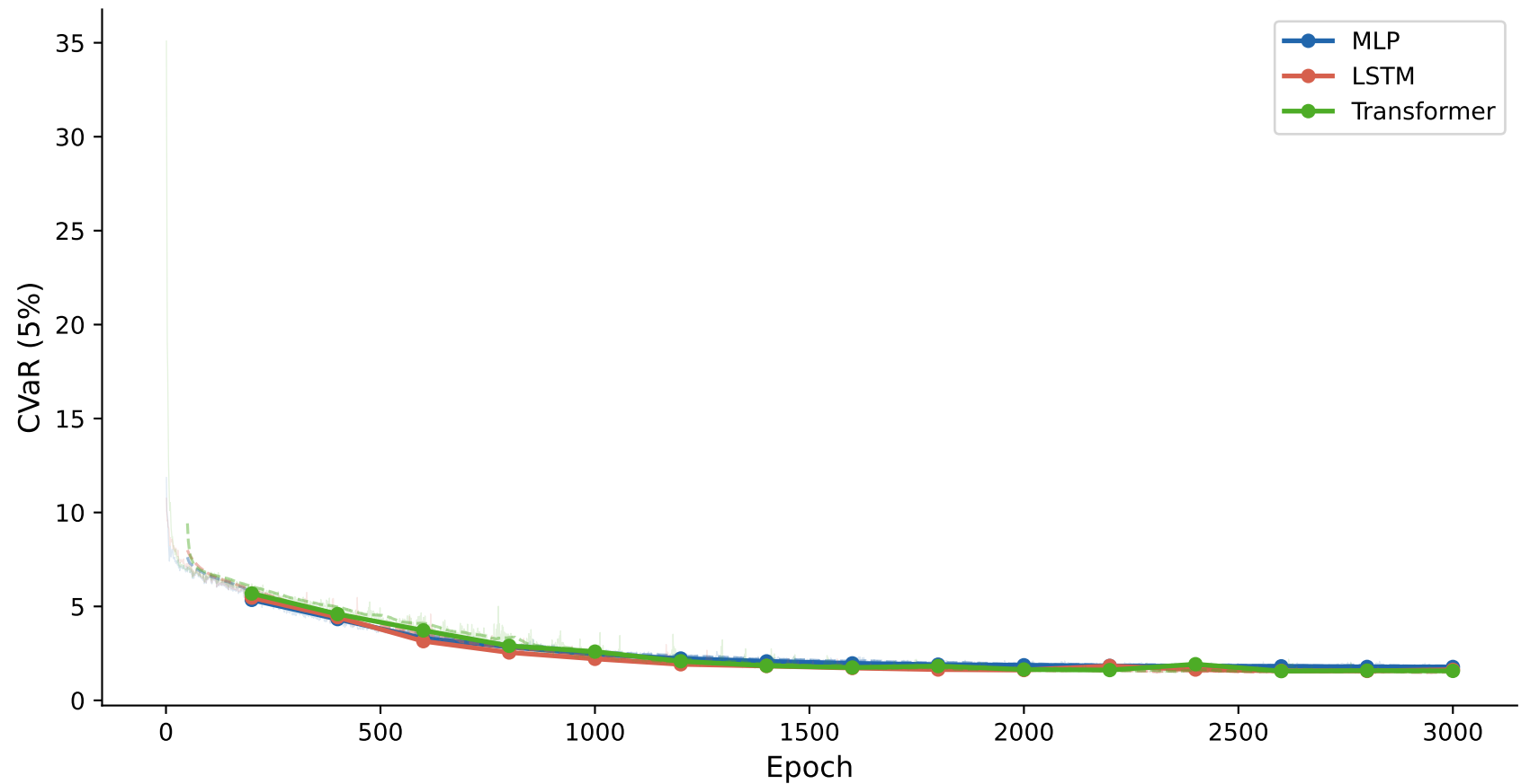
Heston Asian call (REDUCED): CVaR convergence (dashed = train MA-50; solid = eval every 200 epochs)
