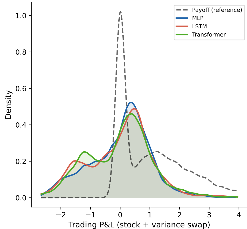
Trading P&amp;L vs Payoff (dashed)
