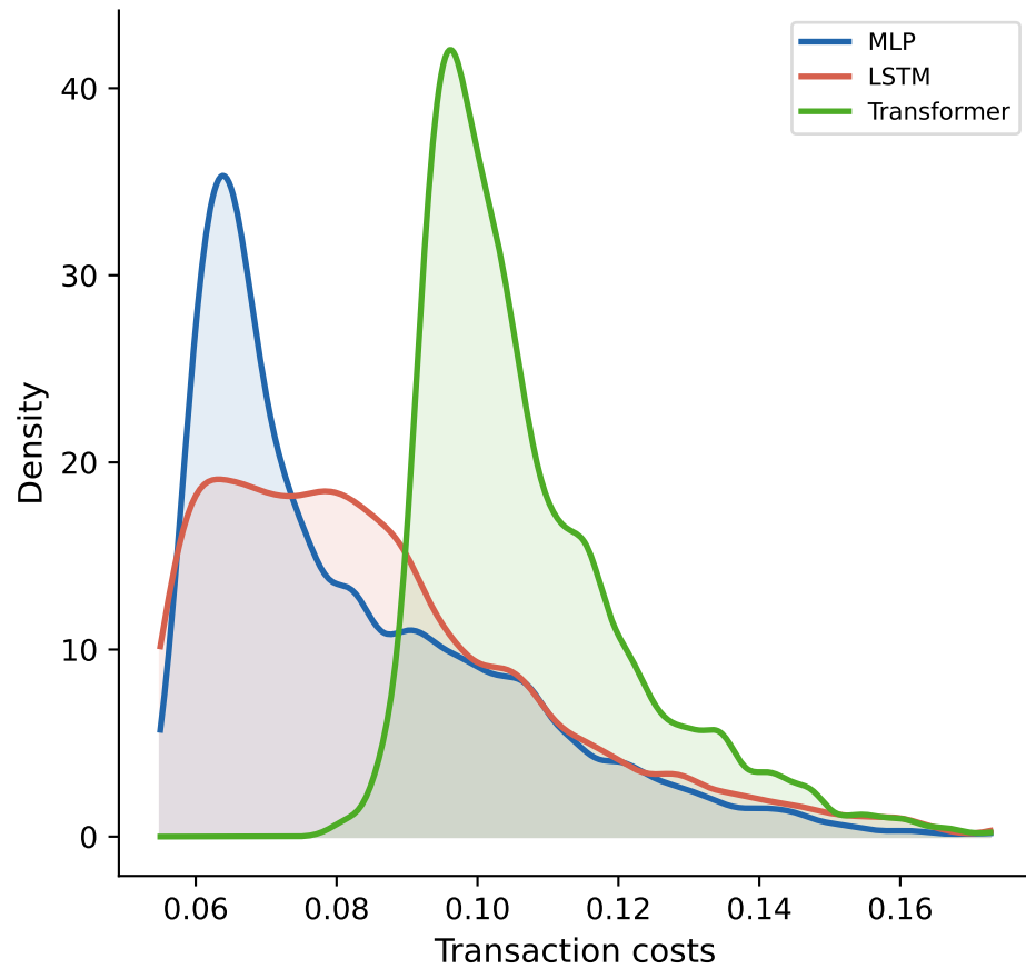
Transaction cost distributions
