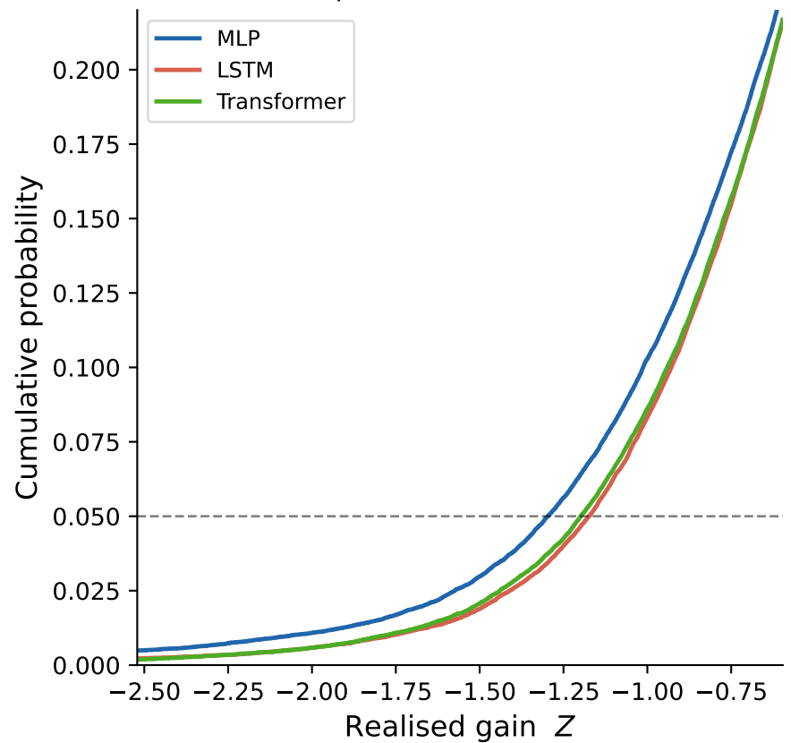
Empirical CDF (tail zoom)
