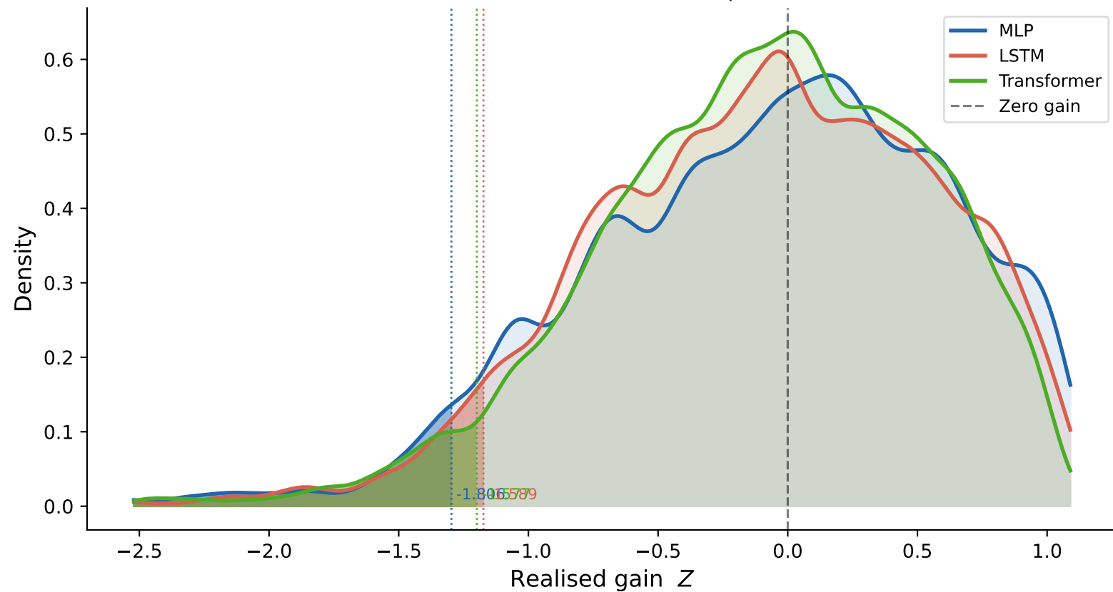
Heston Asian call (REDUCED features): gain distributions (shaded = CVaR tail, dotted = 5th percentile)
