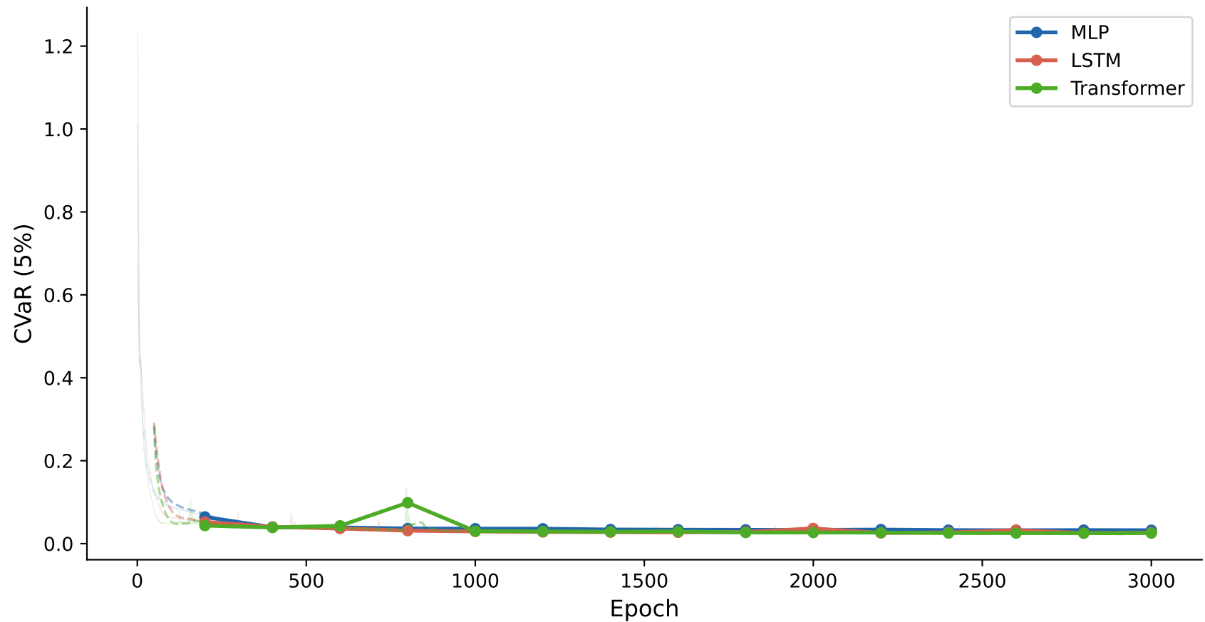
Heston DOC: CVaR convergence (dashed = train MA-50; solid = eval every 200 epochs)
