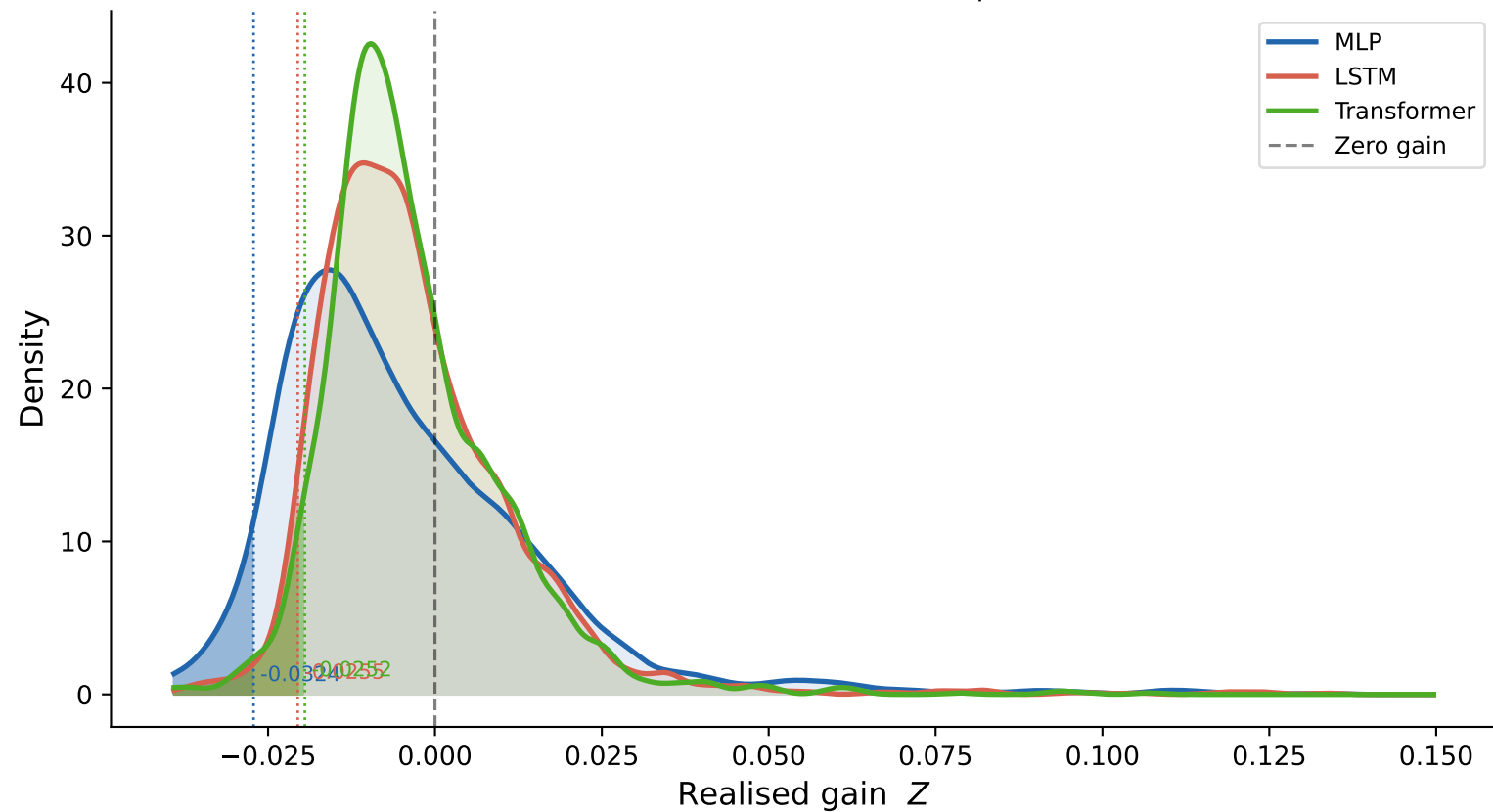
Heston DOC: gain distributions (shaded = CVaR tail, dotted = 5th percentile)
