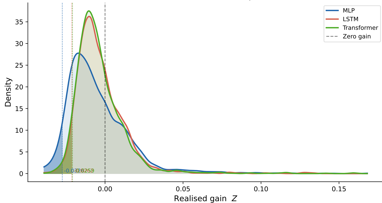
Heston DOC (REDUCED features): gain distributions (shaded = CVaR tail, dotted = 5th percentile)
