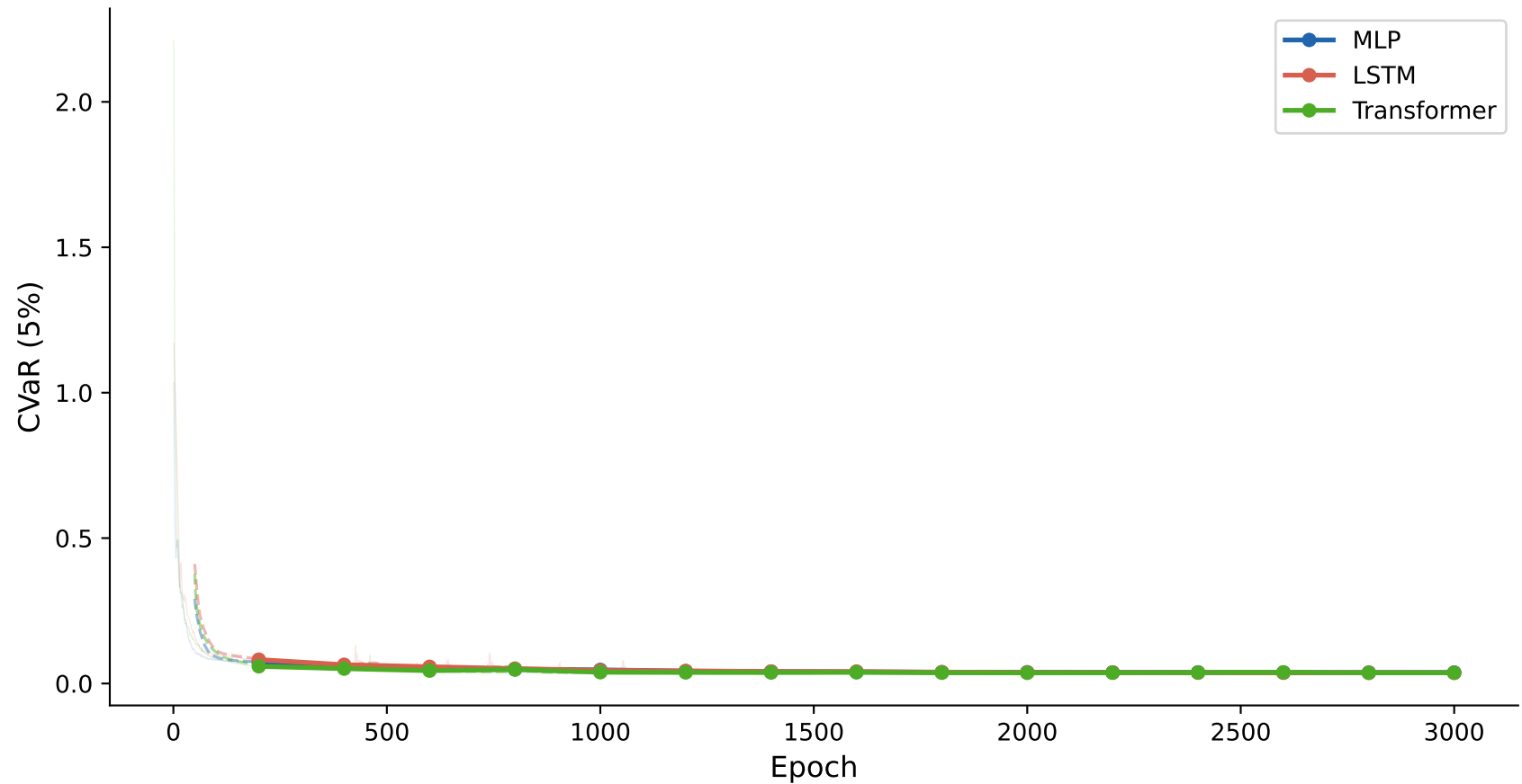
CVaR convergence (dashed = train MA-50; solid = eval every 200 epochs)
